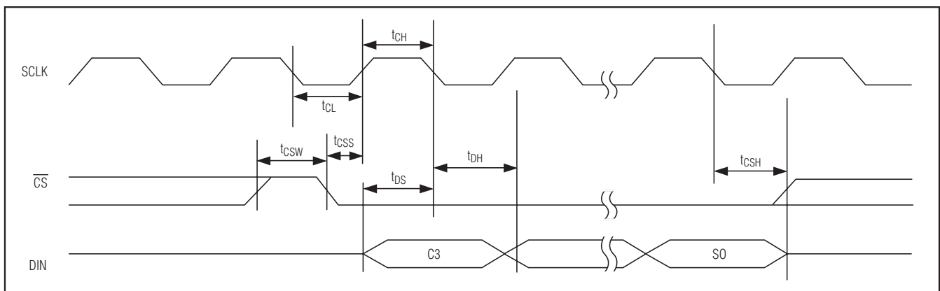
Figure 1. Timing Diagram
