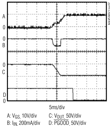
CIRCUIT-BREAKER EVENT ( C_{GATE} = 1000pF , V_{OVERDRIVE} = 20mV )
