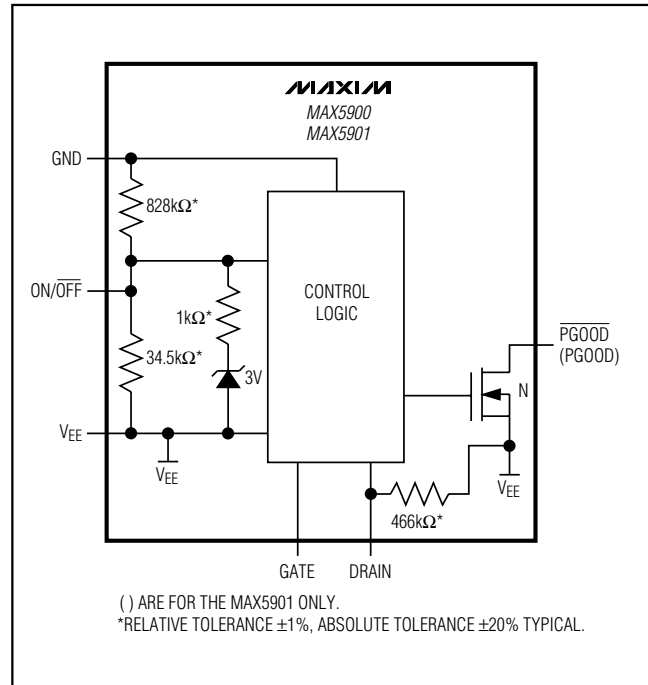
Figure 1. Functional Diagram
