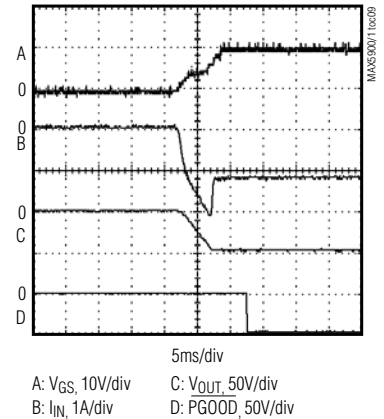
STARTUP WAVEFORMS ( R_L = 40\Omega , C_L = 100\mu F )
