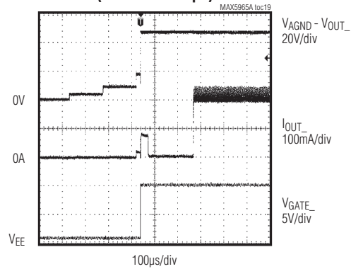
STARTUP WITH VALID PD (25k \Omega AND 0.1µF)
