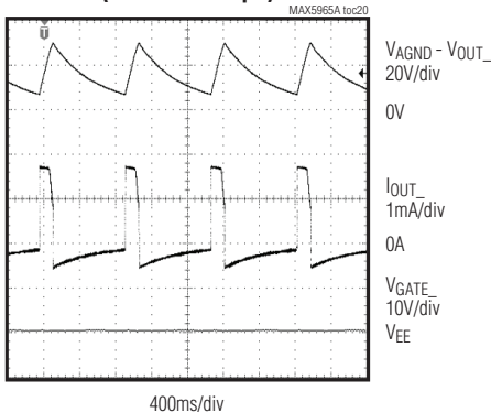
DETECTION WITH INVALID PD (25k \Omega AND 10µF)
