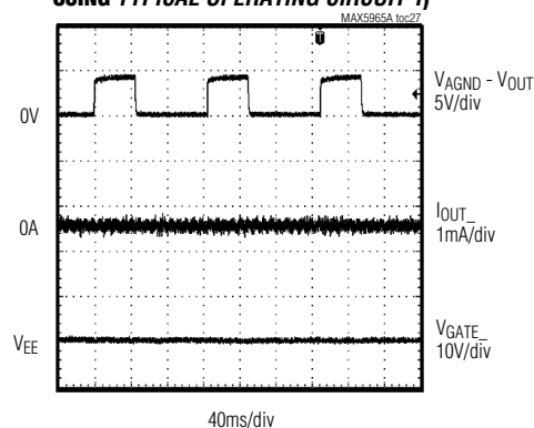
DETECTION WITH INVALID PD (OPEN CIRCUIT, USING TYPICAL OPERATING CIRCUIT 1)
