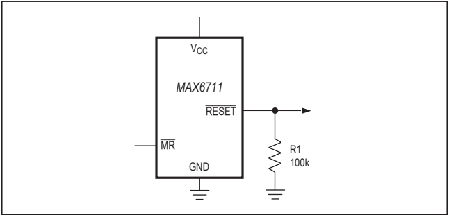
Figure 2. \overline{\text{RESET}} Valid to V_{\text{CC}} = Ground Circuit
