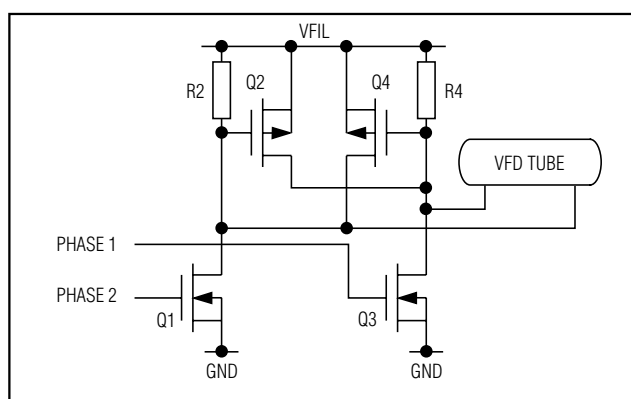
Figure 14. Filament Bridge Driver (MOSFET)
