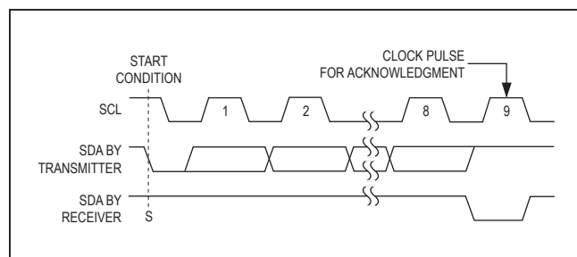
Figure 4. Acknowledge
