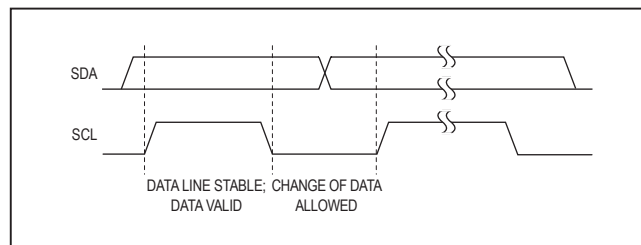
Figure 3. Bit Transfer
