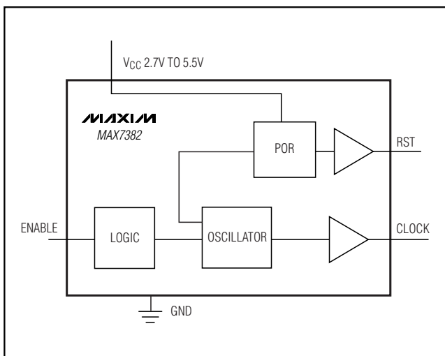
Figure 1. Functional Diagram
