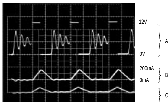
MAX738A/MAX744A SWITCHING WAVEFORMS, DISCONTINUOUS CONDITION
