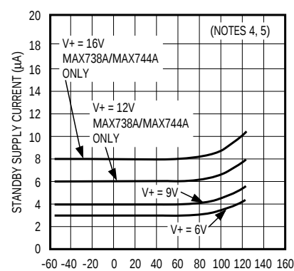
STANDBY SUPPLY CURRENT vs. TEMPERATURE
