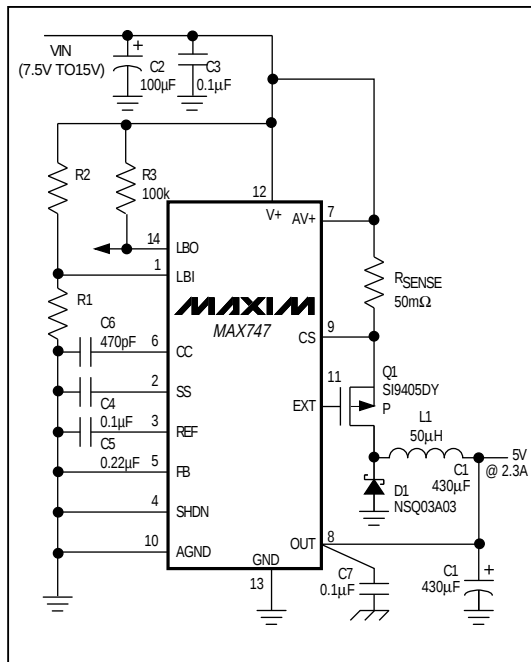
Figure 1a. +5V Standard Application Circuit
