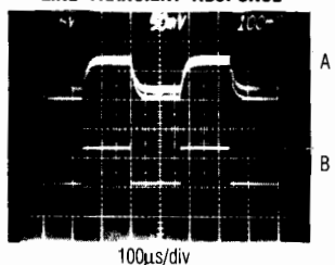
MAX752 LINE TRANSIENT RESPONSE
