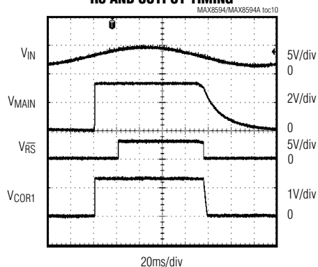
RS AND OUTPUT TIMING
