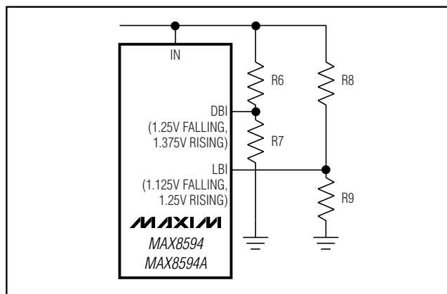
Figure 5. Setting the DBI and LBI Thresholds with Four Resistors
