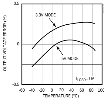
MAX866 OUTPUT VOLTAGE ERROR vs. TEMPERATURE
