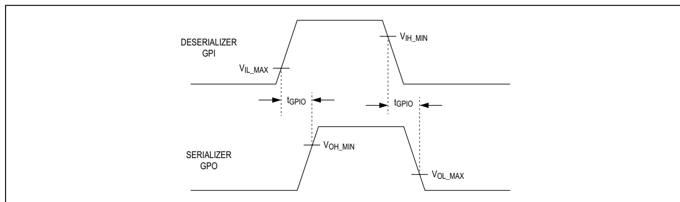
Figure 9. GPI-to-GPO Delay
