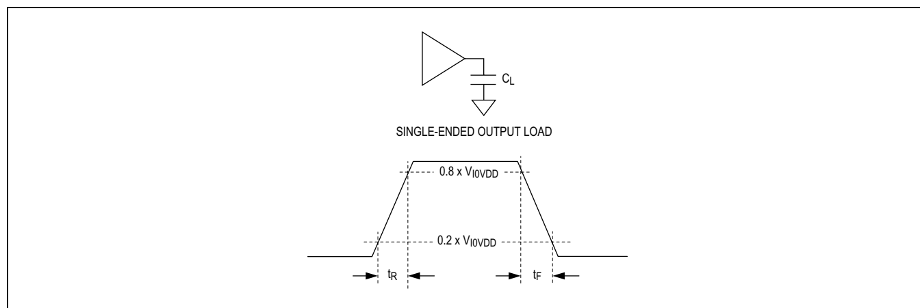
Figure 7. Output Rise-and-Fall Times
