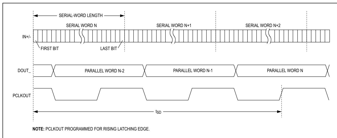
Figure 8. Deserializer Delay
