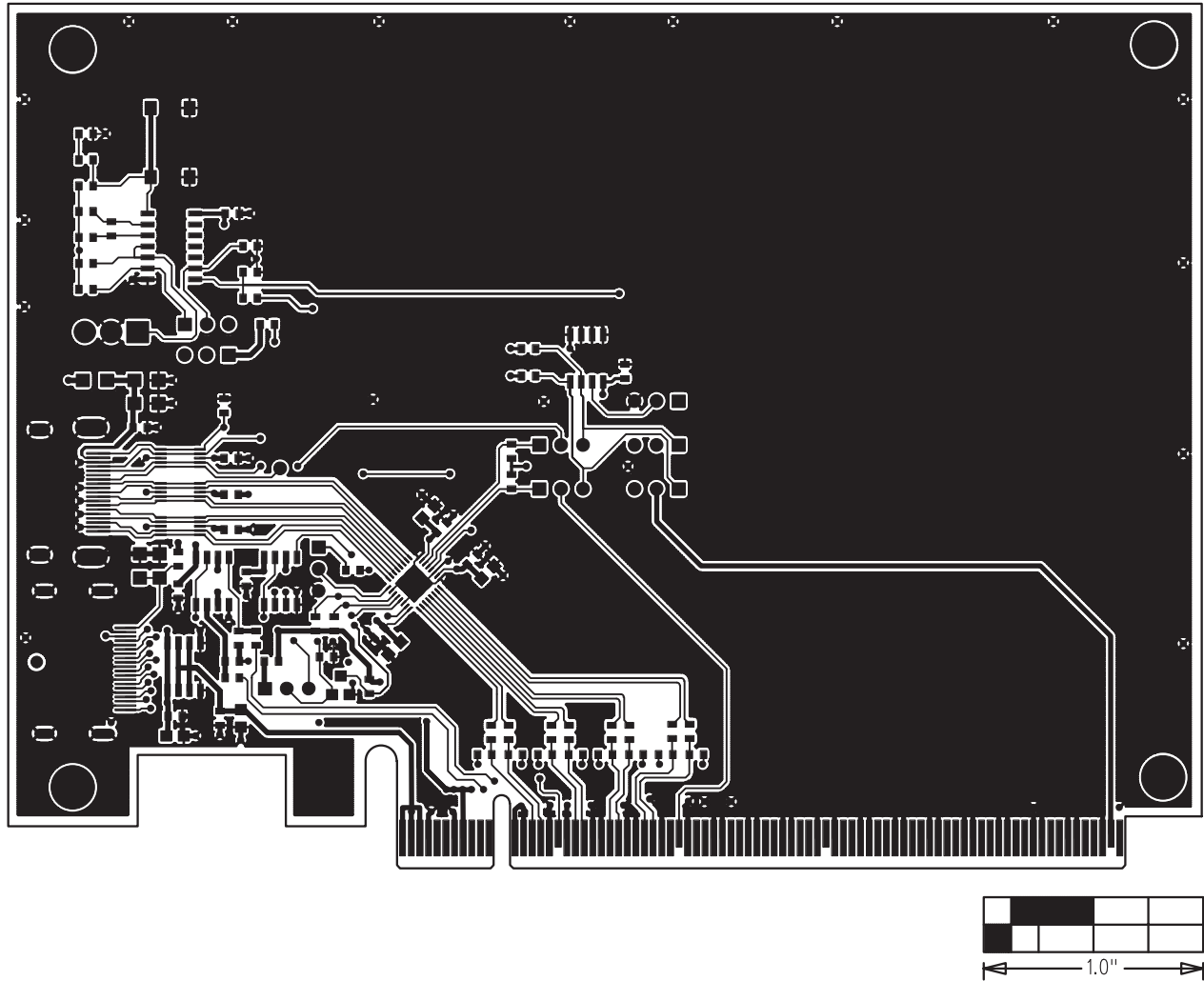
Figure 3. MAX9406 EV Kit PCB Layout—Component Side
