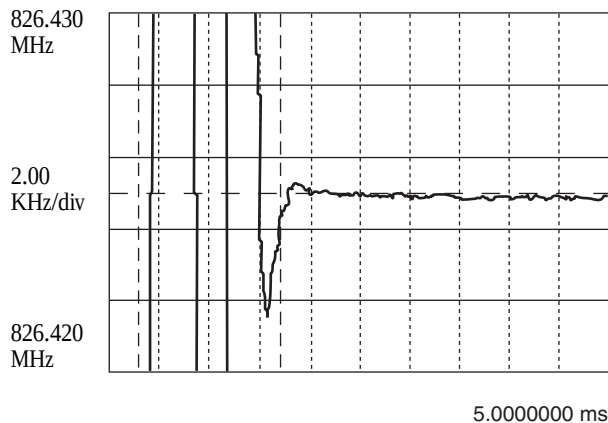
PLL Lock Up Time = 1.4 ms (810.425 MHz \rightarrow 826.425 MHz, within \pm 1 \text{ kHz} )
