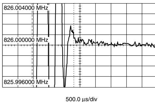
PLL Lock Up Time = 1.3 ms (810.000 MHz → 826.000 MHz, within \pm 1 \text{ kHz} )
