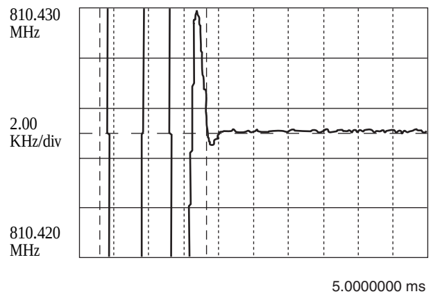
PLL Lock Up Time = 1.52 ms (826.425 MHz \rightarrow 810.425 MHz, within \pm 1 \text{ kHz} )
