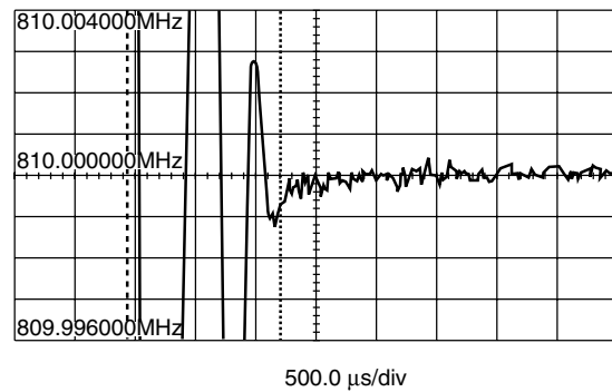
PLL Lock Up Time = 1.28 ms (826.000 MHz → 810.000 MHz, within \pm 1 \text{ kHz} )
