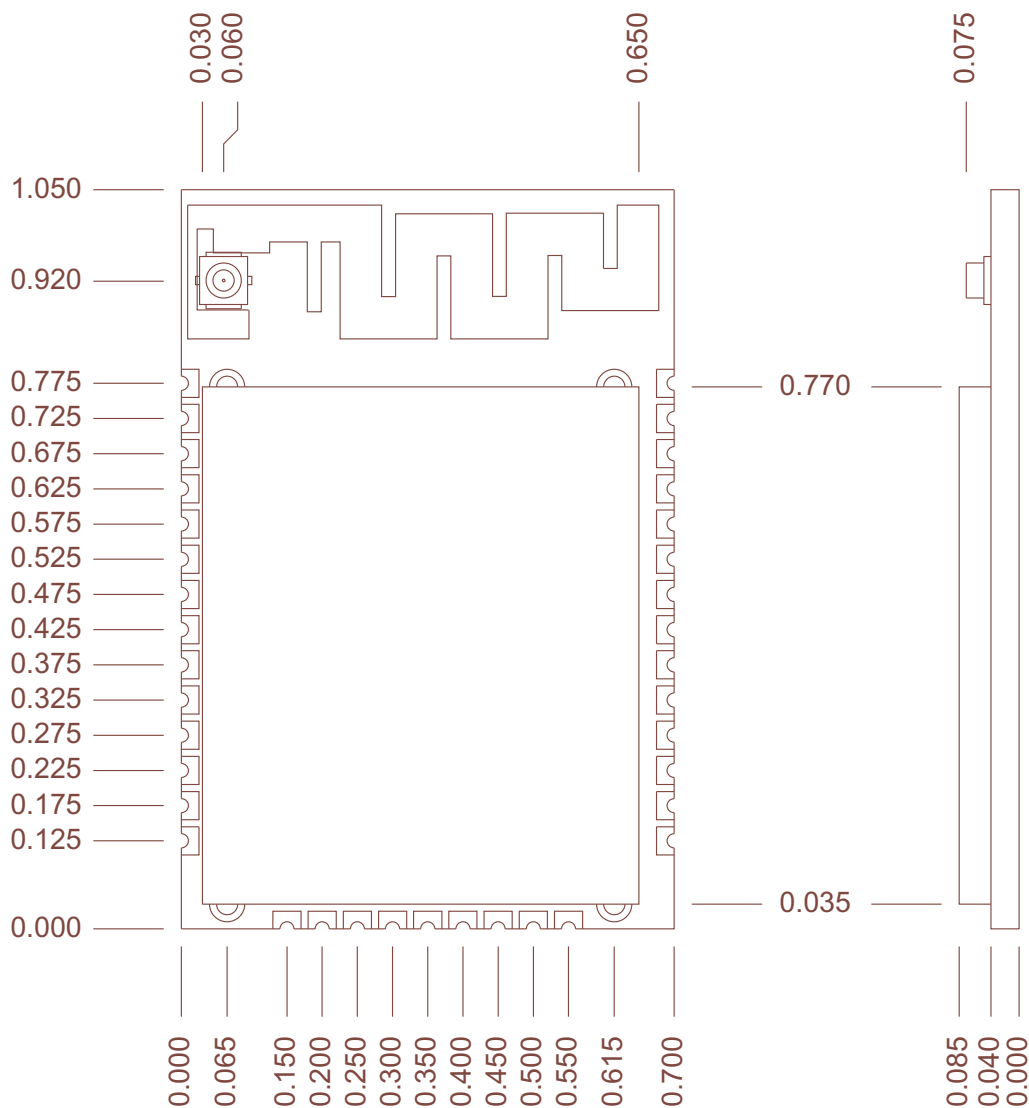
FIGURE 1-3: MRF24WN0MA/MB MODULE PHYSICAL DIMENSIONS (TOP AND SIDE VIEW)
