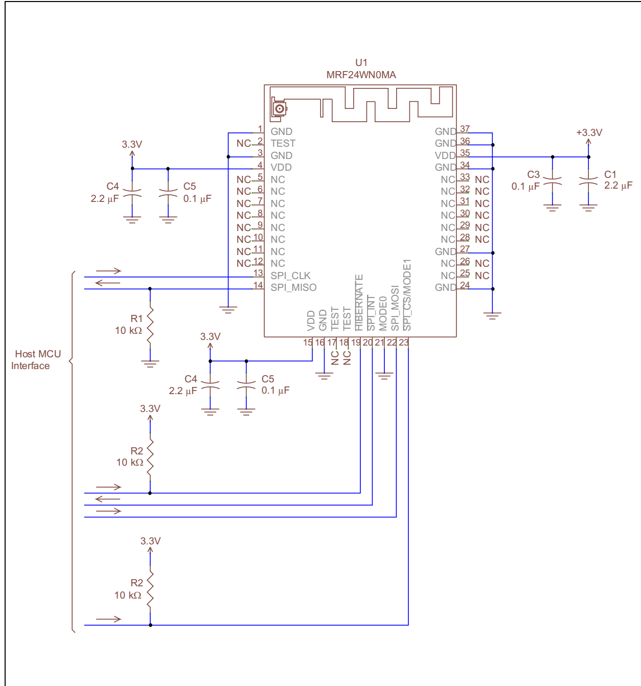
FIGURE 3-1: APPLICATION SCHEMATIC
