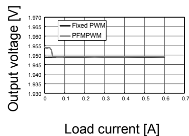
Load regulation
