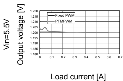
Load regulation
