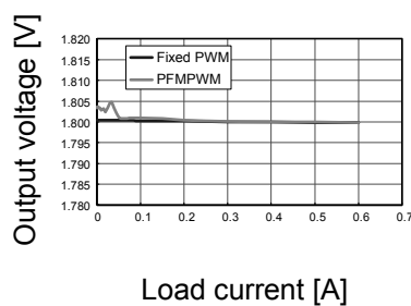
Load regulation
