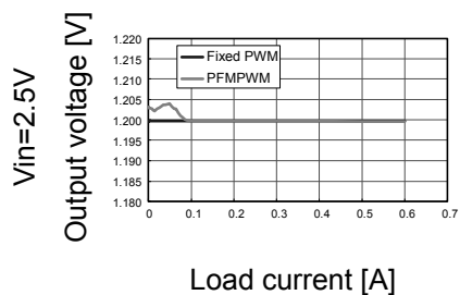
Load regulation
