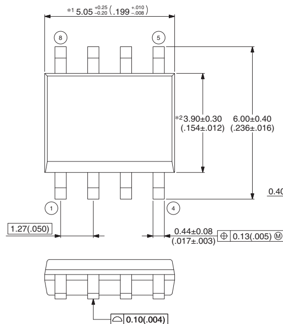
8-pin plastic SOP (FPT-8P-M02)
