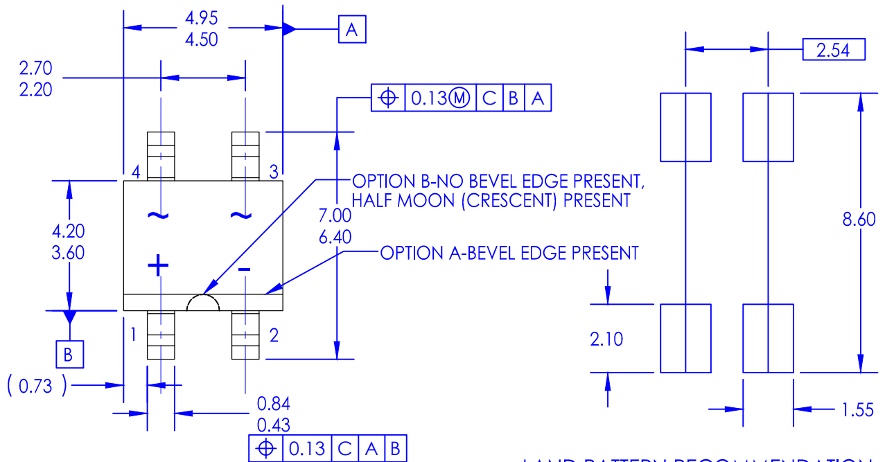
LAND PATTERN RECOMMENDATION
