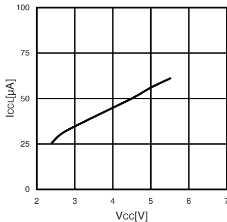
I_{CCL} - V_{CC} T_A = +25^\circ\text{C} , FMP=16 kHz (divided by 2) Subclock mode with the external clock operating
