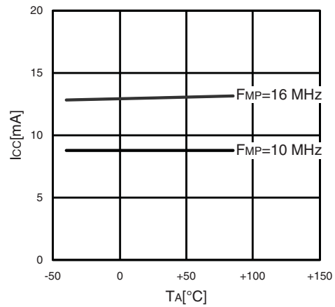
I_{CCS} - T_A V_{CC} = 5.5\text{ V} , FMP=10, 16 MHz (divided by 2) Main sleep mode with the external clock operating
