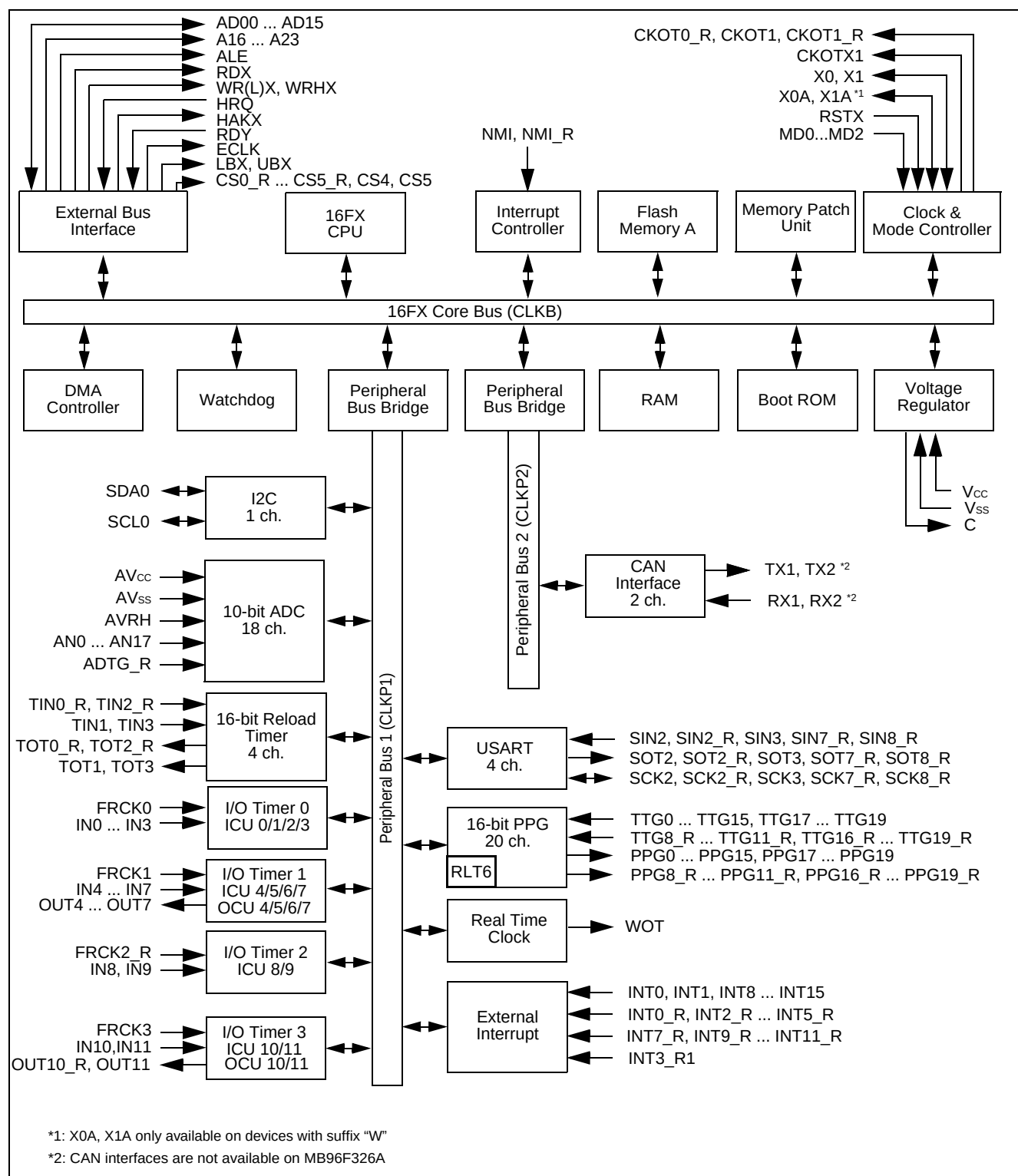
Block diagram of MB96(F)32x
