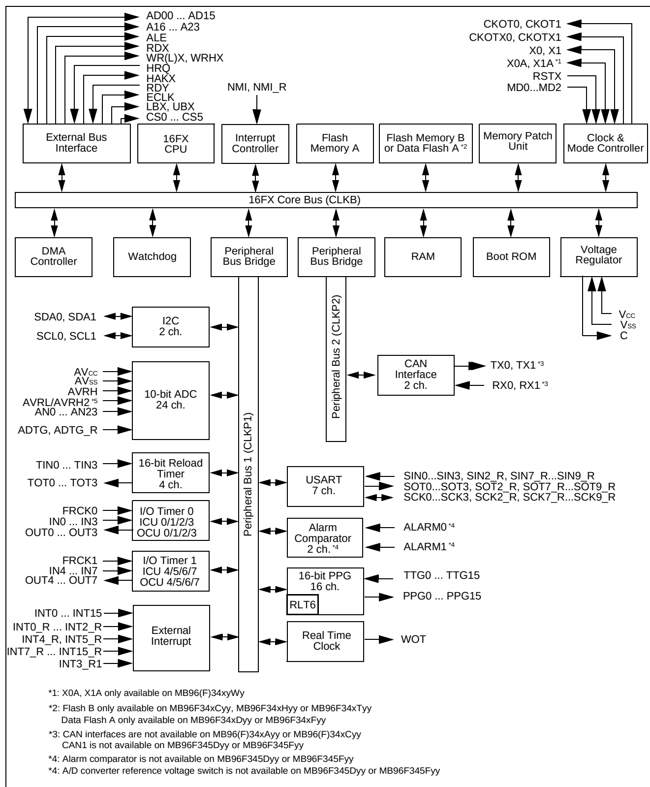
Block diagram of MB96(F)34x
