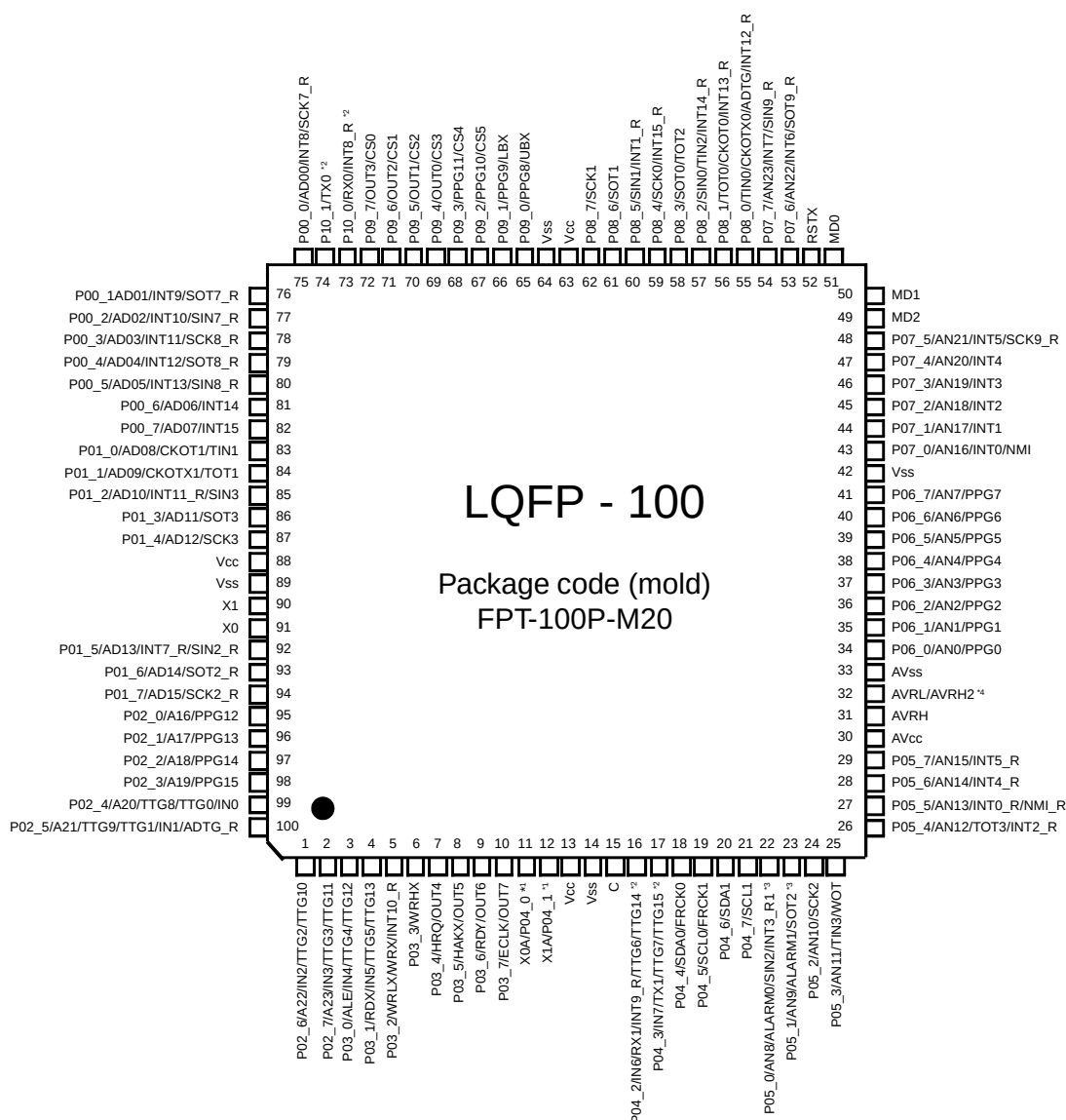
Pin assignment of MB96(F)34x (FPT-100P-M20)
