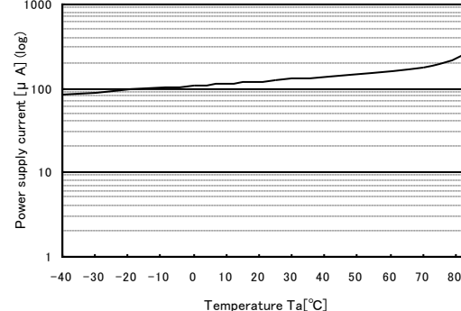
Iccs sleep operation(sub oscillation) temperature characteristics(semi-log) Vcc:5.5V, Peripheral:32KHz
