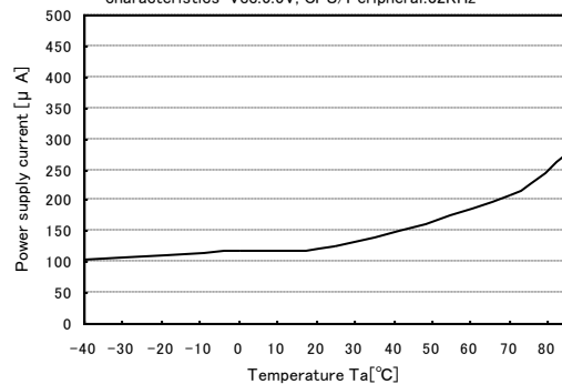
Icc normal operation(sub oscillation) temperature characteristics Vcc:5.5V, CPU/Peripheral:32KHz
