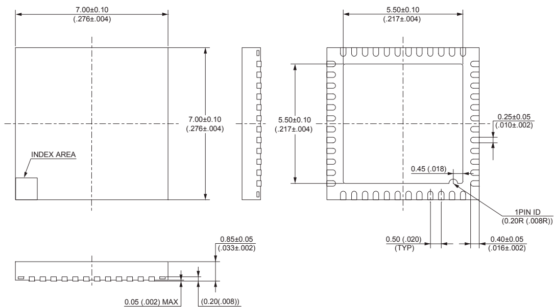
48-pin plastic QFN (LCC-48P-M73)
