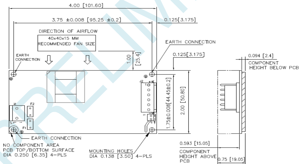
Mechanical Drawing – Option 1 without PGPF
