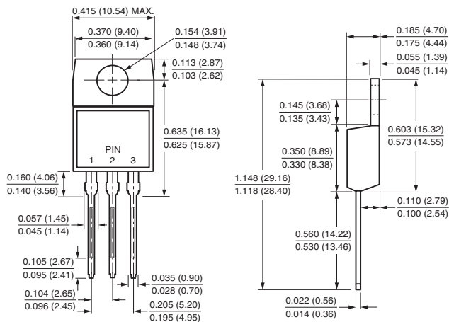
TO-220AB
