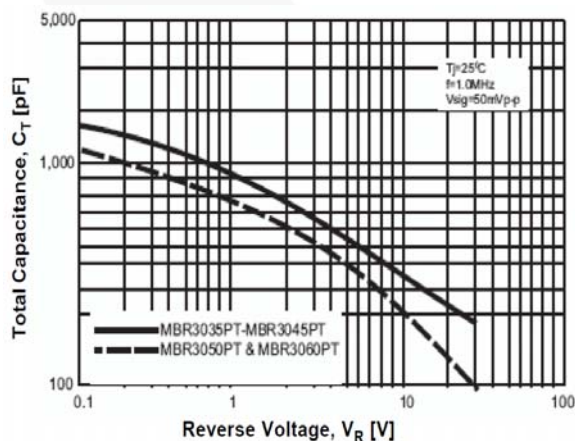
Figure 5. Total Capacitance
