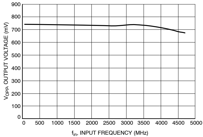
Figure 4. Input Frequency (f in ) versus Output Voltage (V Opp )
