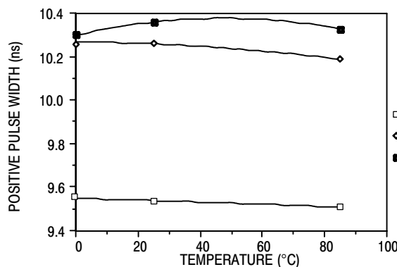
Figure 7. MC10H642 Positive PW versus Temperature, V_{CC} = 5.0\text{ V}
