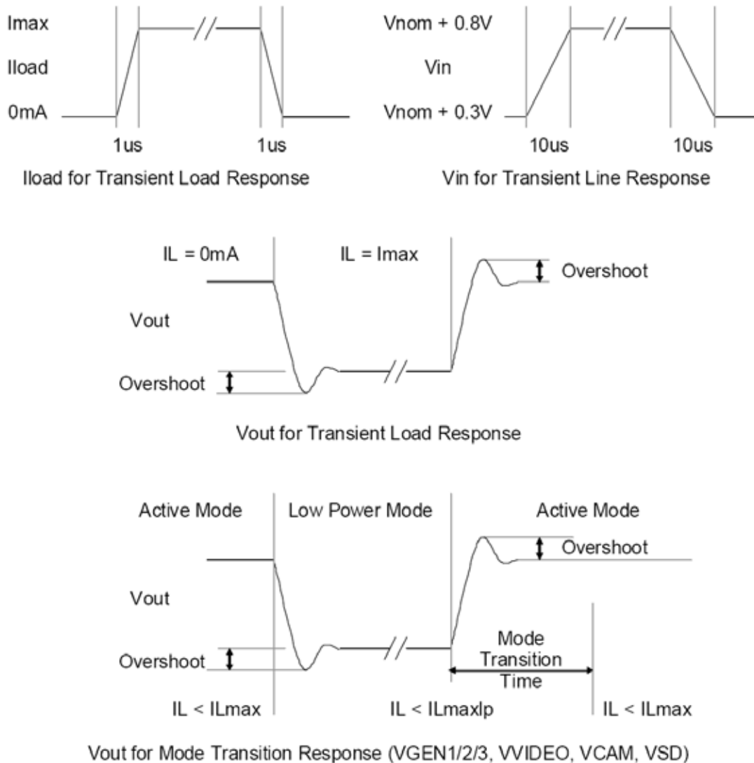
Figure 25. Transient Waveforms
