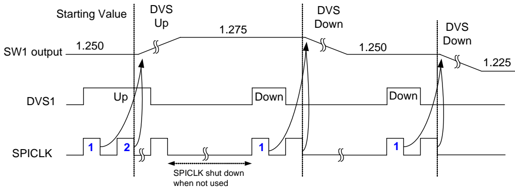
Figure 21. SID Control Example for Increment & Decrement
