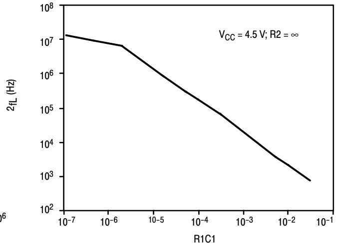
Figure 21. Typical Frequency Lock Range (2f L ) versus R1C1
