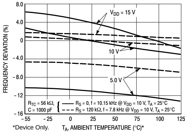
Figure 2. RC Oscillator Stability
