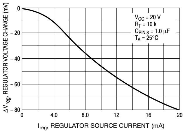
Figure 10. Regulator Output Voltage Change versus Source Current
