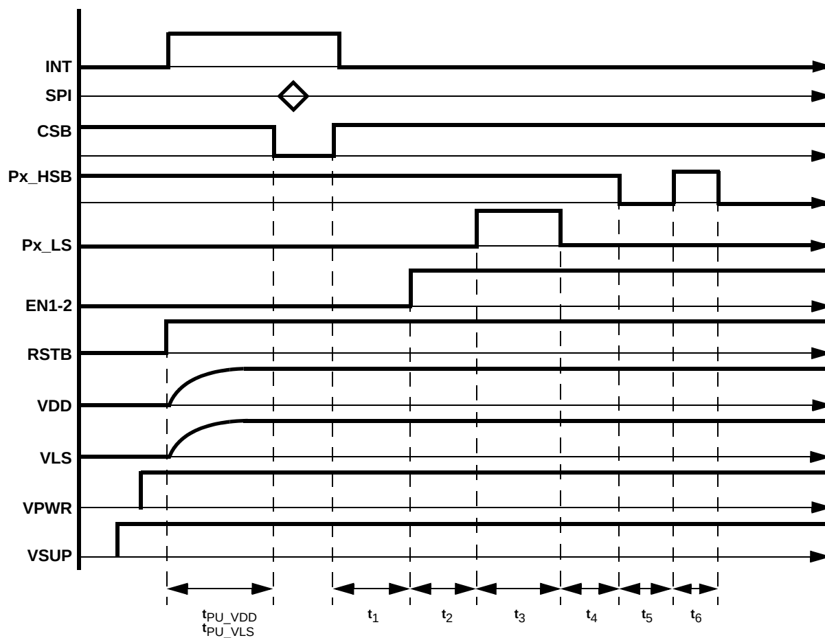
Figure 19. Full Initialization
