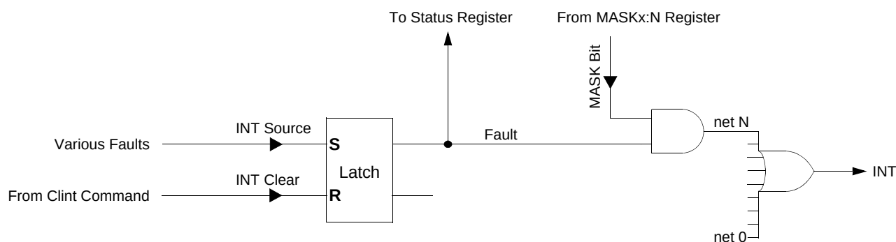
Figure 17. Interrupt Handling
