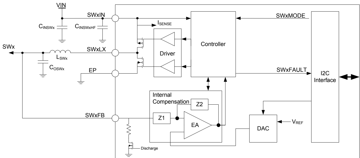
Figure 8. Generic SWx Block Diagram
