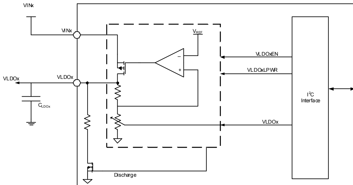
Figure 10. General LDO Block Diagram
