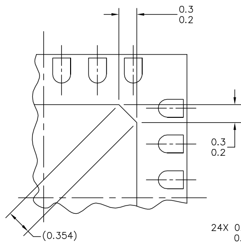
DETAIL M PIN 1 BACKSIDE IDENTIFIER
