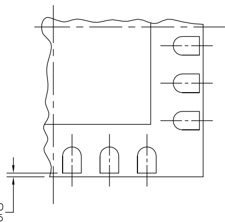
DETAIL N CORNER CONFIGURATION
