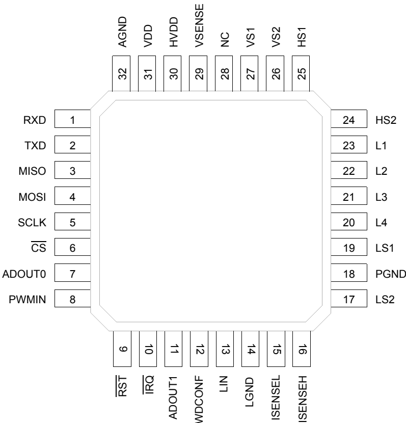
Figure 3. 33912 Pin Connections
