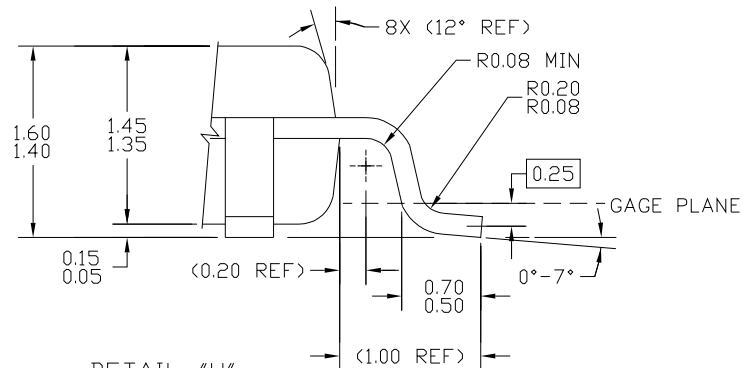
DETAIL "H"
