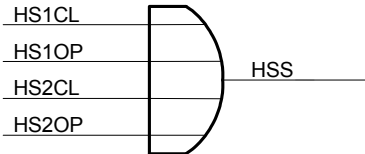
Figure 46. High-side Status
