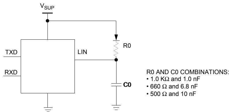
Figure 5. Test Circuit for Transient Test Pulses (Lx)
