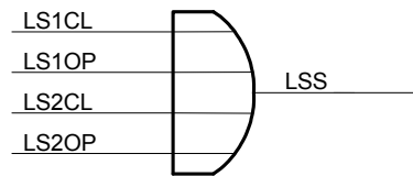
Figure 24. Low-side Status
