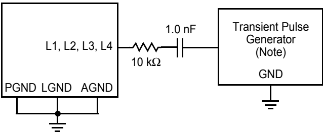
Figure 27. Test Circuit for Transient Test Pulses (LIN)
