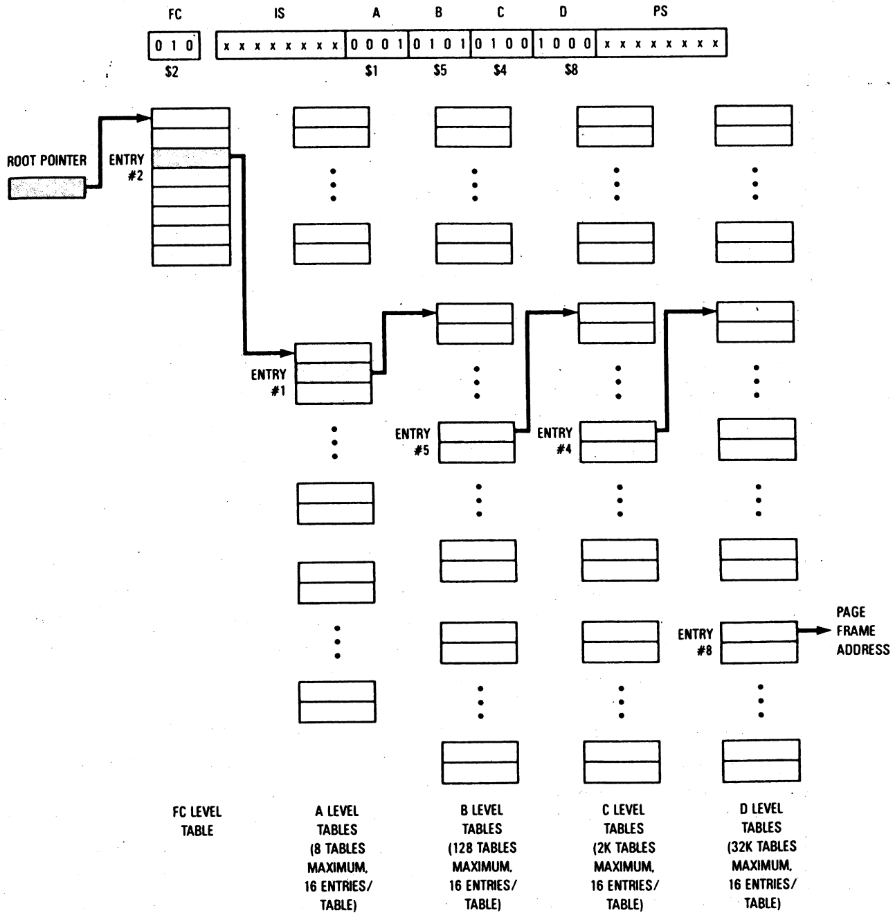
Figure 9-20. Five-Level Table Search
