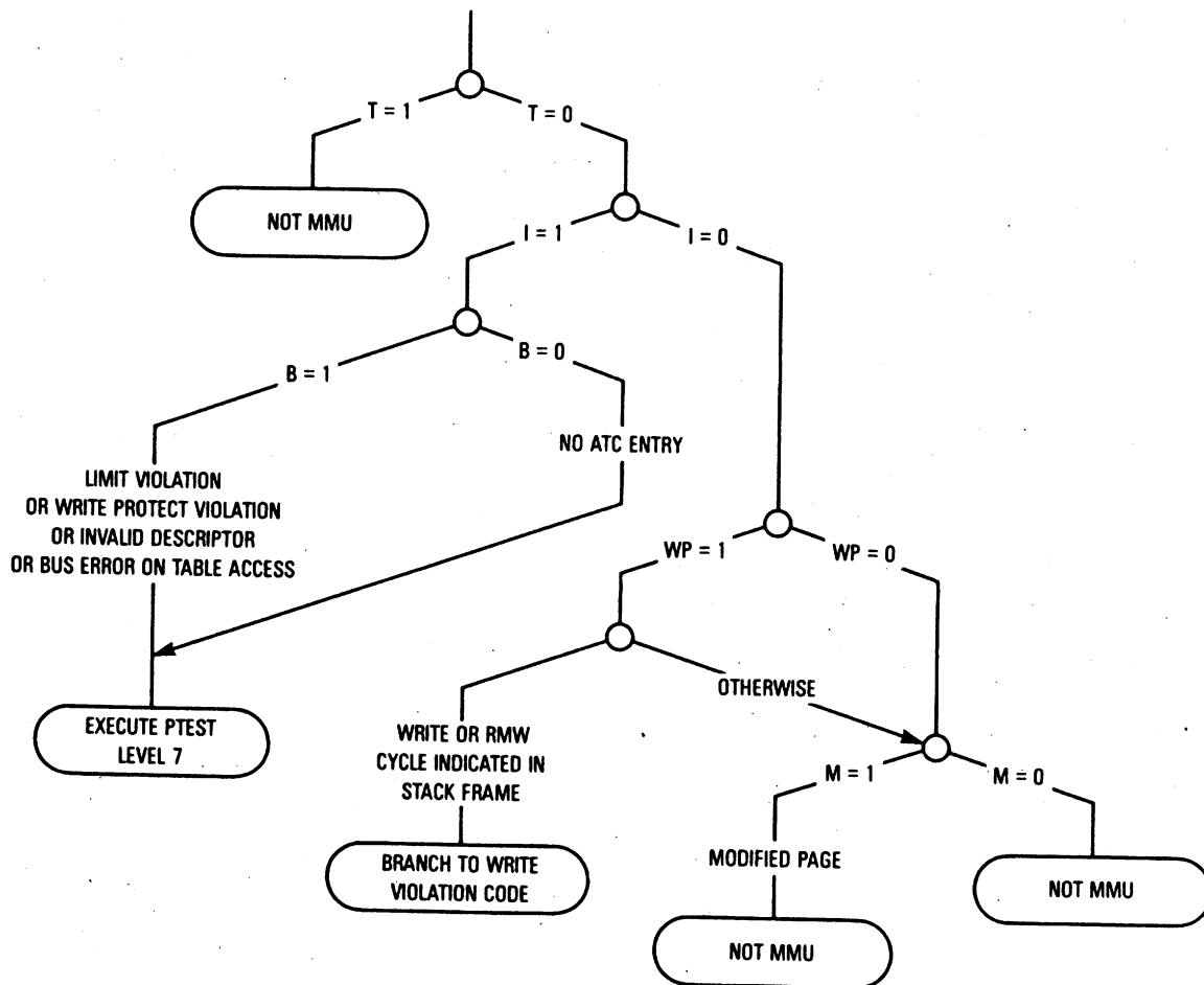
Figure 9-39. MMU Status Interpretation PTEST Level 0
