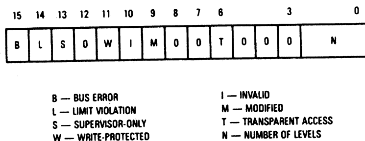
Figure 9-38. MMU Status Register (MMUSR) Format
