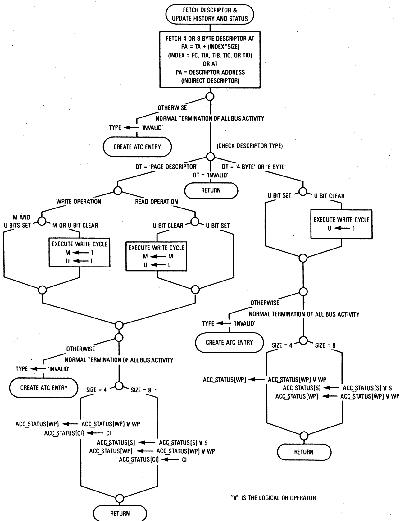
Figure 9-29. Detailed Flowchart of Descriptor Fetch Operation
