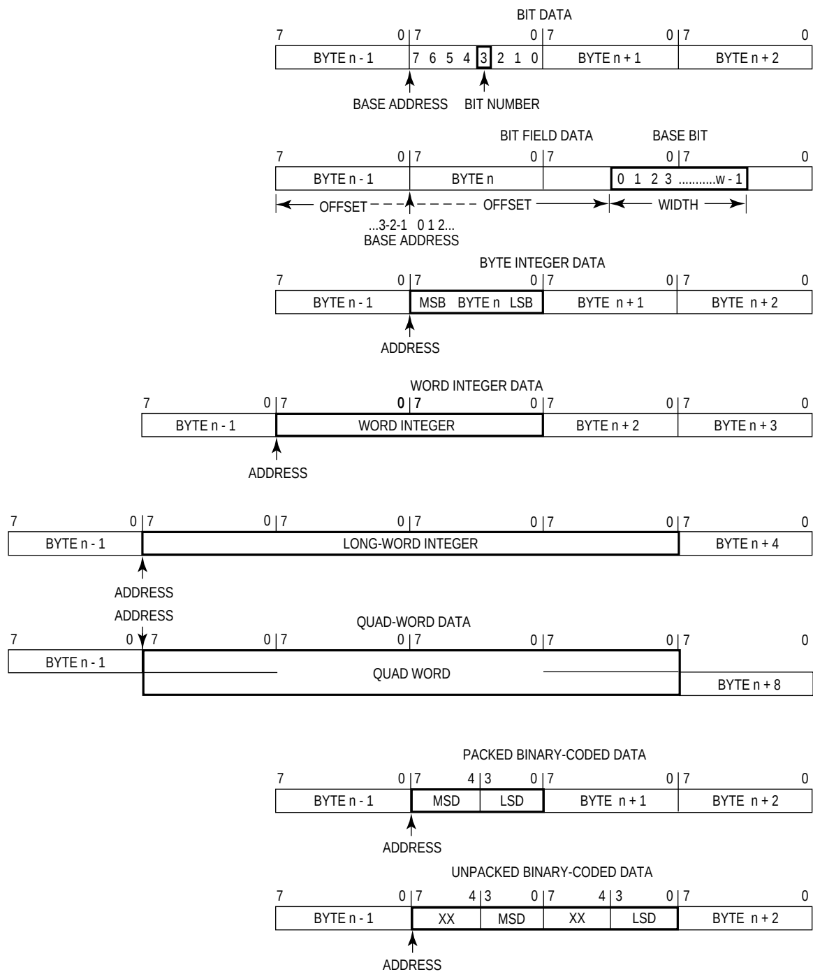
Figure 2-2. Memory Data Organization
