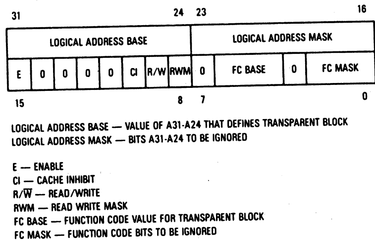
Figure 9-37. Transparent Translation Register (TT0 and TT1) Format
