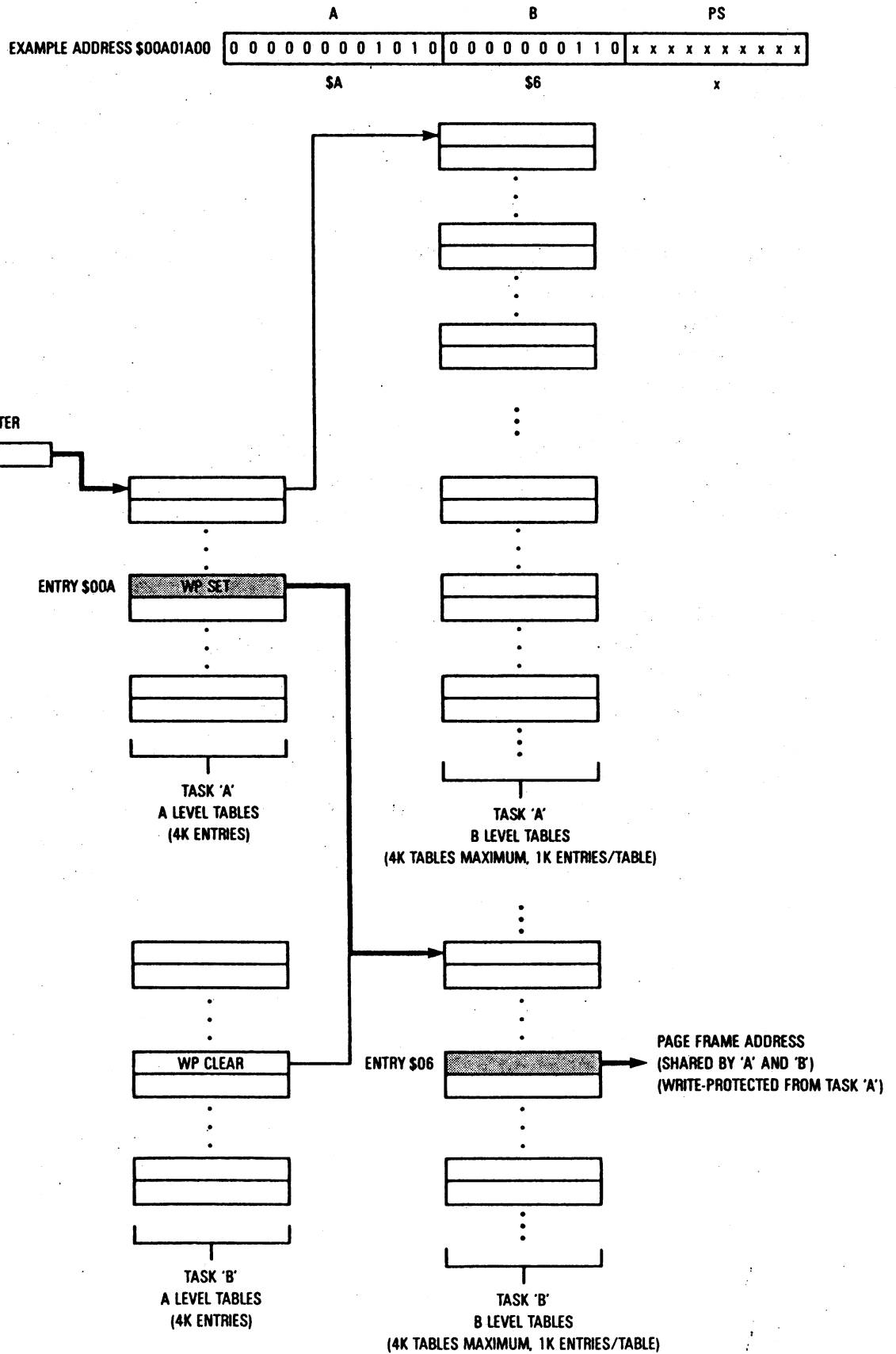
Figure 9-23. Example Translation Tree Using Shared Tables
