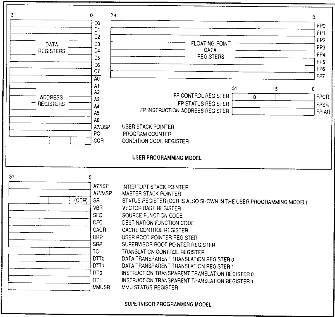
Figure 1-2. Programming Model
