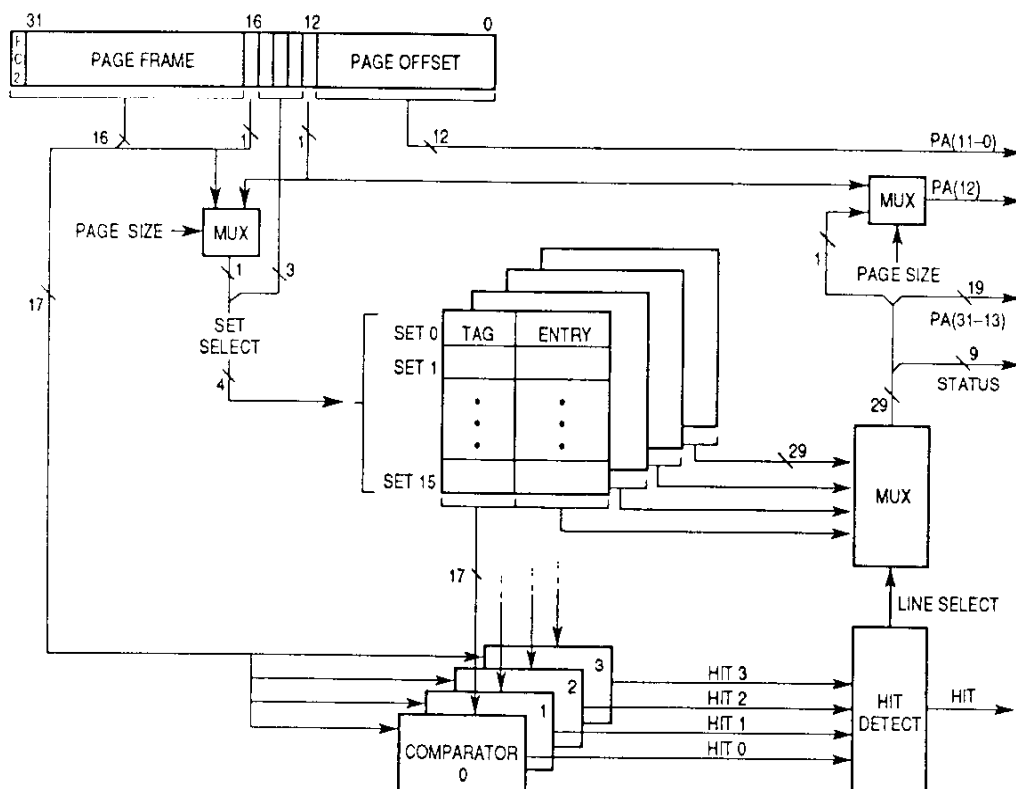
Figure 3-20. ATC Organization
