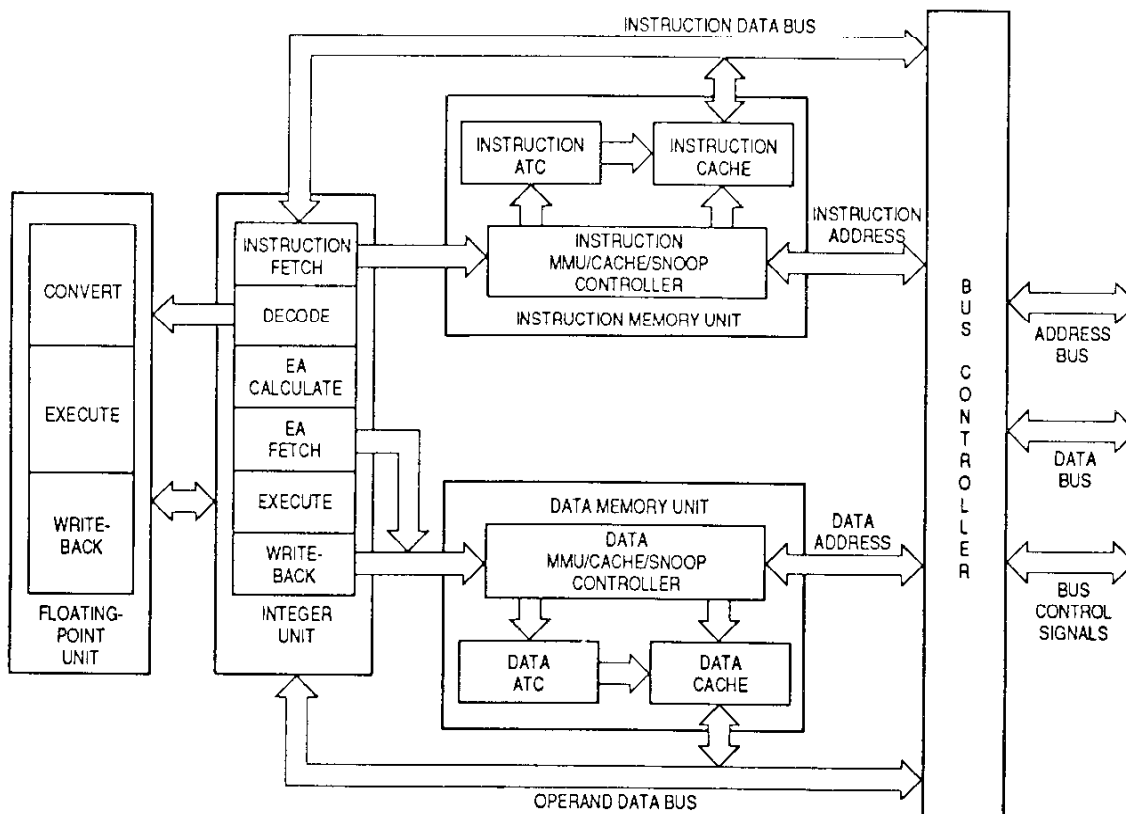
Figure 1-1. Block Diagram
