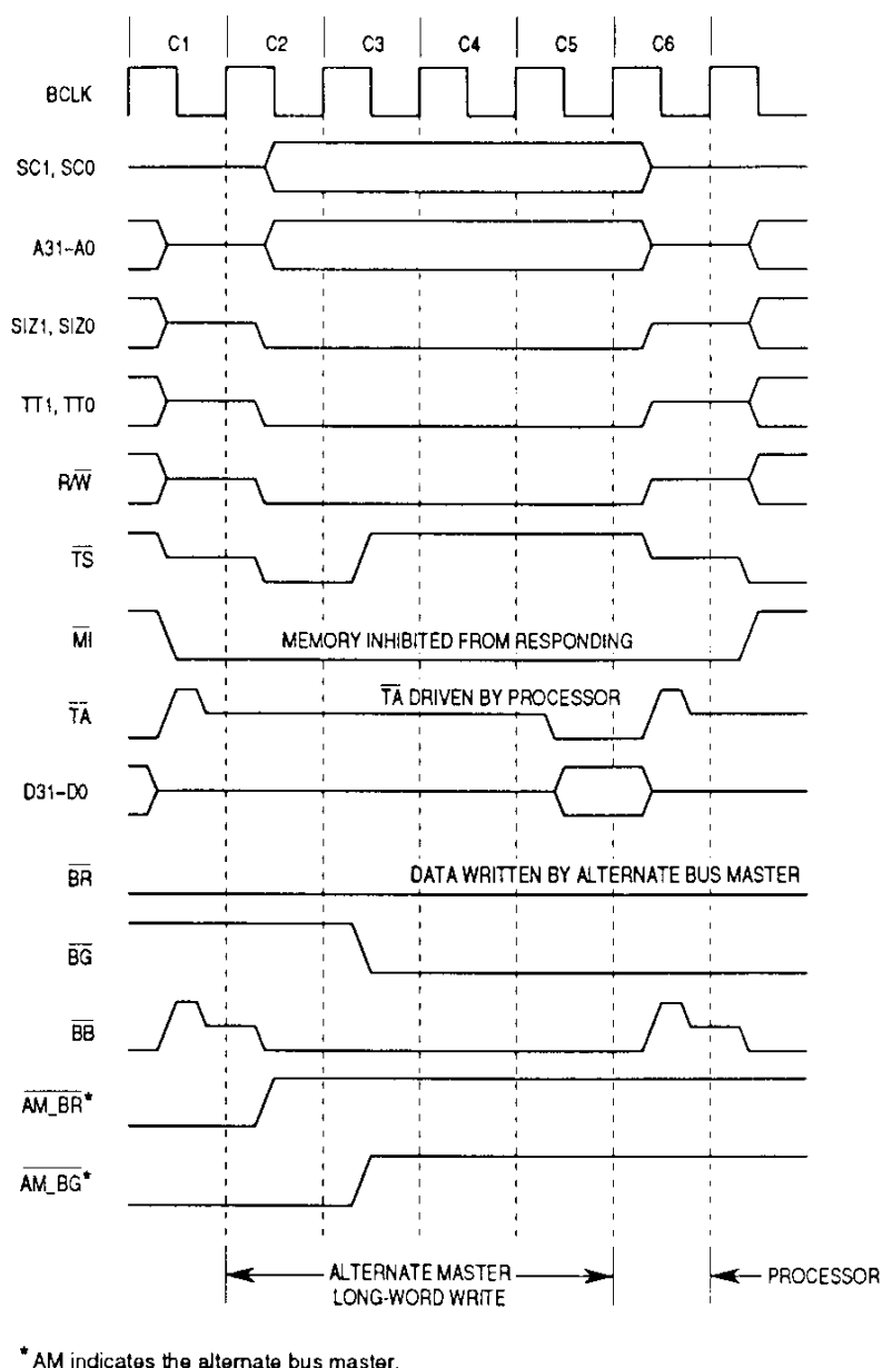
Figure 7-43. Snooped Long-Word Write, Memory Inhibited
