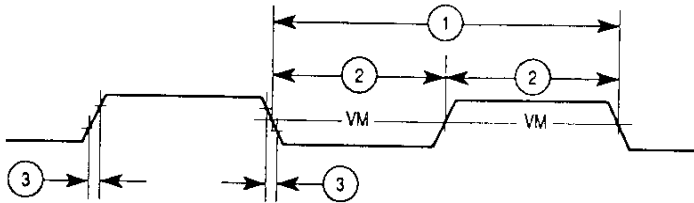
Figure 6-8. Clock Input Timing Diagram
