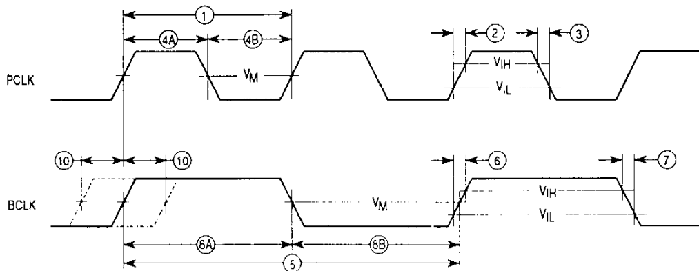
Figure 11-1. Clock Input Timing Diagram
