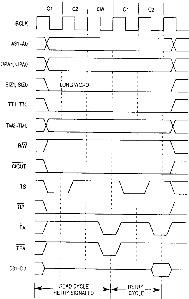
Figure 7-28. Retry Read Transfer Timing
