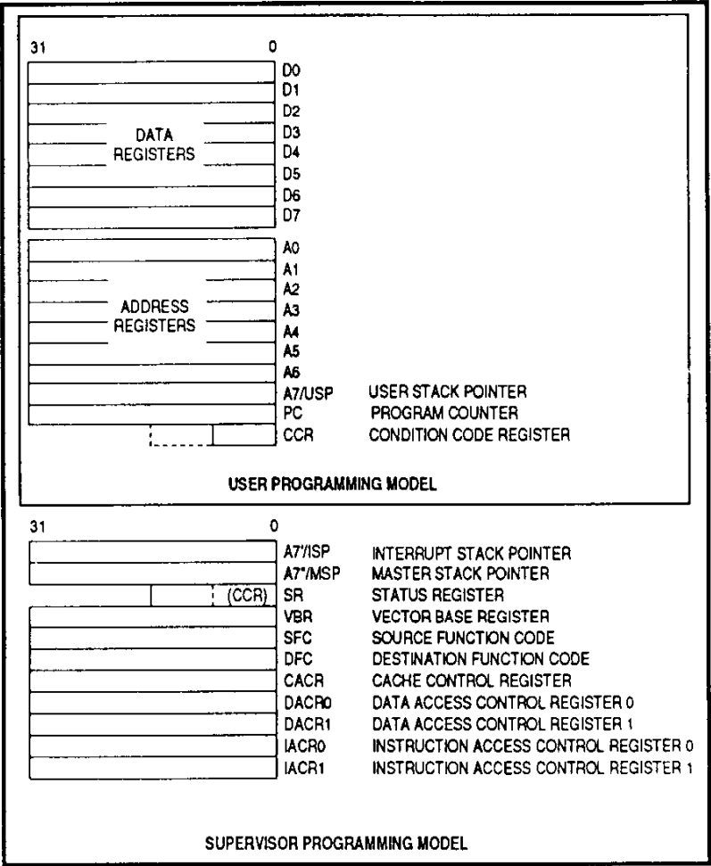
Figure B-2. MC68EC040 Programming Model
