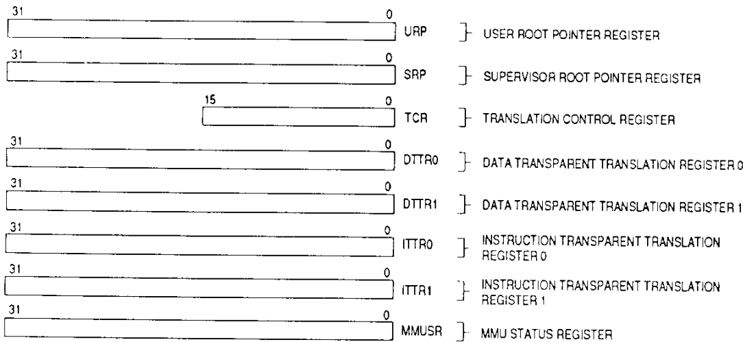
Figure 3-2. Memory Management Programming Model
