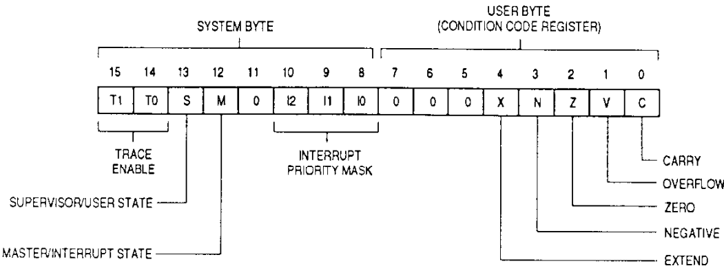
Figure 2-5. Status Register
