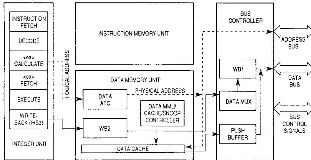
Figure 2-2. Write-Back Cycle Block Diagram
