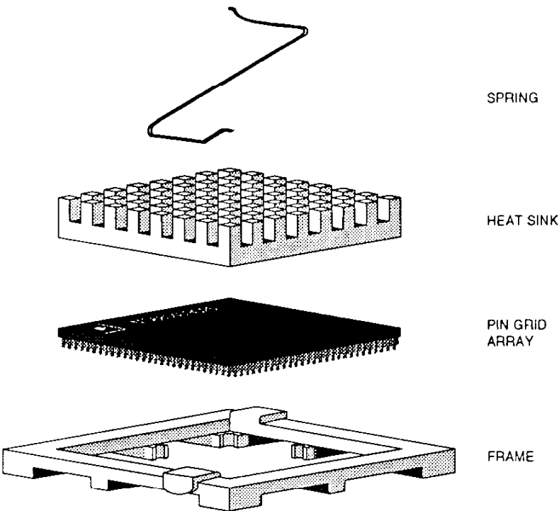
Figure 11-11. Heat Sink with Attachment
