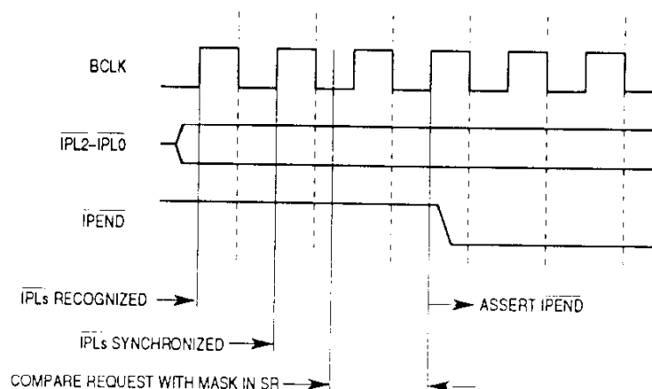
Figure 7-20. Assertion of \overline{IPEND}
