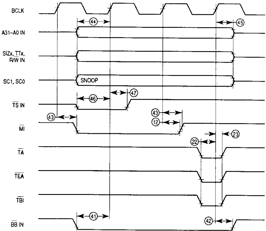
Figure C-16. Snoop Miss Timing
