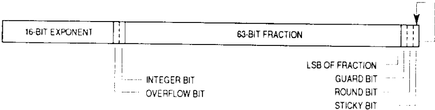
Figure 9-7. Intermediate Result Format
