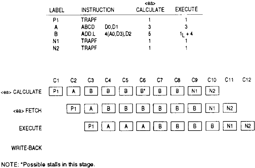
Figure 10-3. Interlocked Stages
