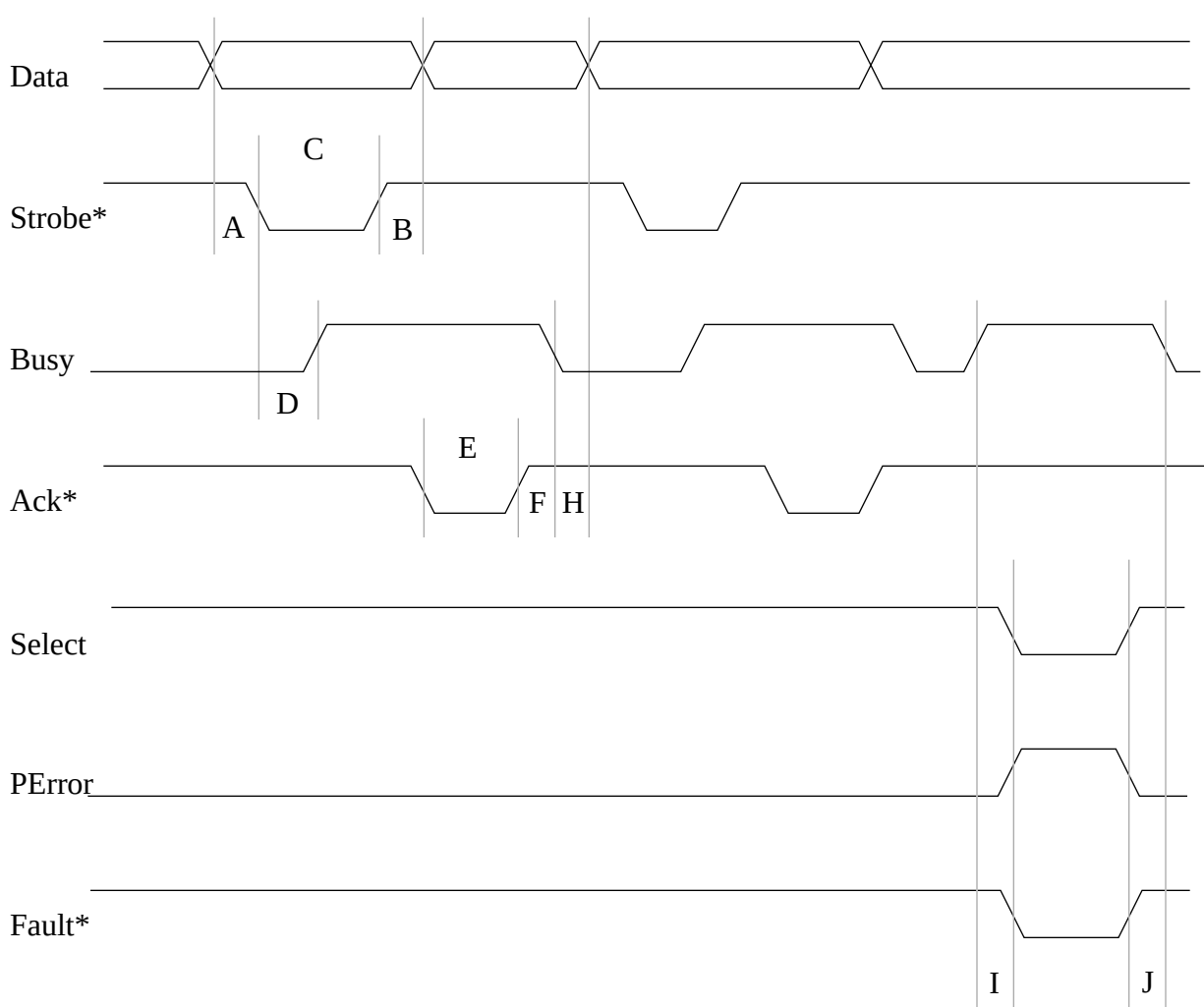
Figure 7-94. Centronics Interface Signals
