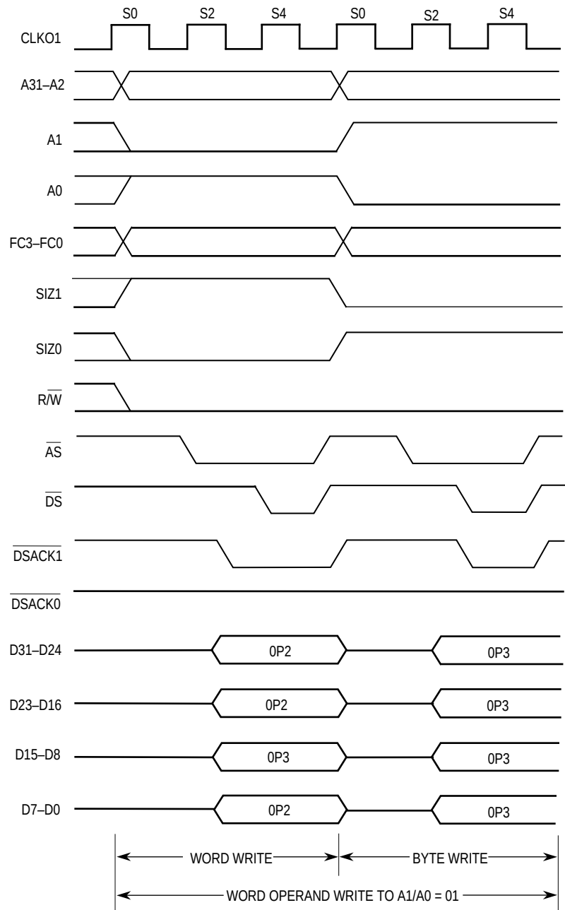
Figure 4-11. Misaligned Word Transfer to Word Port Timing
