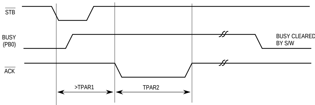
Figure 7-92. Centronics Receiver Timing Mode 3
