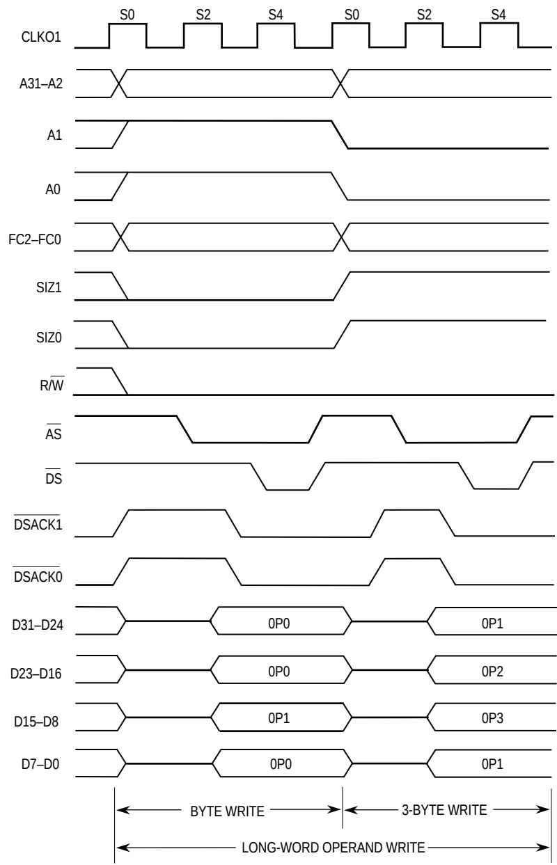
Figure 4-13. Misaligned Long-Word Transfer to Long-Word Port Timing
