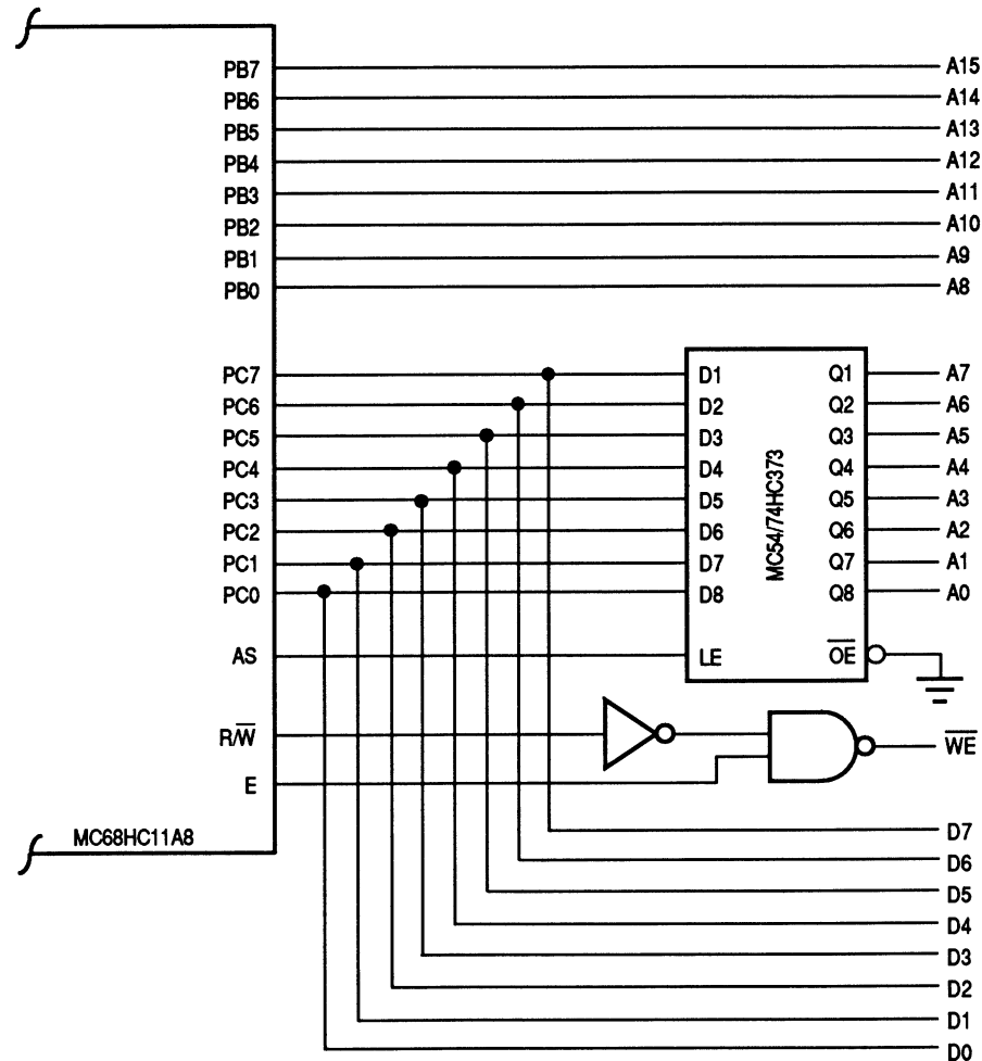
Address/Data Demultiplexing
