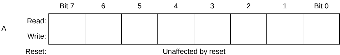
Figure 10-2. Accumulator (A)
