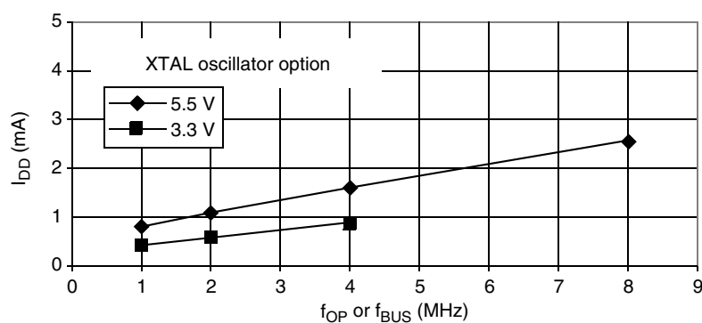
Figure 17-7. Typical Wait Mode I_{DD} (XTAL osc), with All Modules Turned Off (25 °C)
