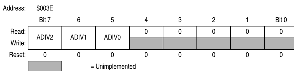
Figure 10-5. ADC Input Clock Register (ADICLK)
