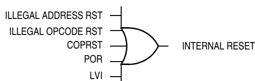
Figure 5-6. Sources of Internal Reset
