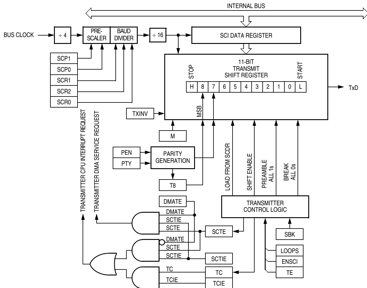
Figure 9-4. SCI Transmitter
