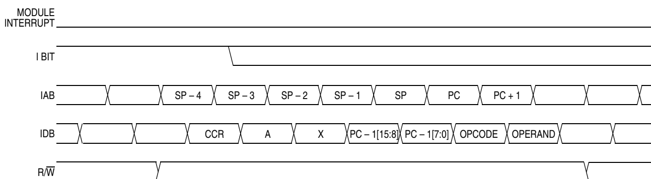
Figure 5-10. Interrupt Recovery
