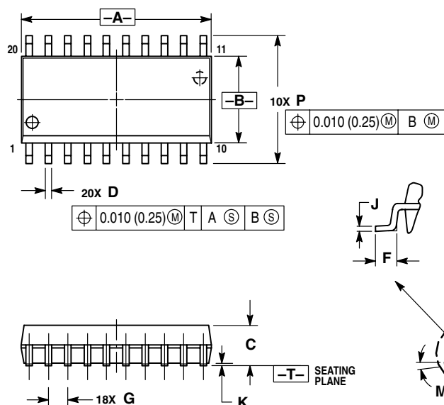
Figure 18-2. 20-Pin SOIC (Case #751D)
