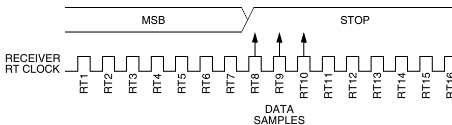
Figure 9-7. Slow Data
