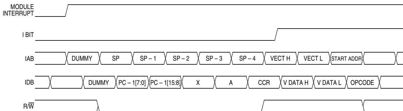
Figure 5-9. Interrupt Entry
