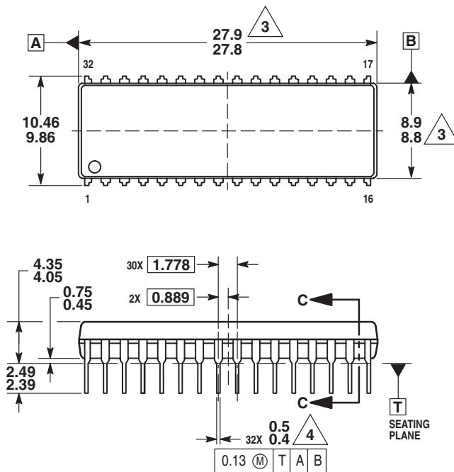
Figure 18-5. 32-Pin SDIP (Case #1376)
