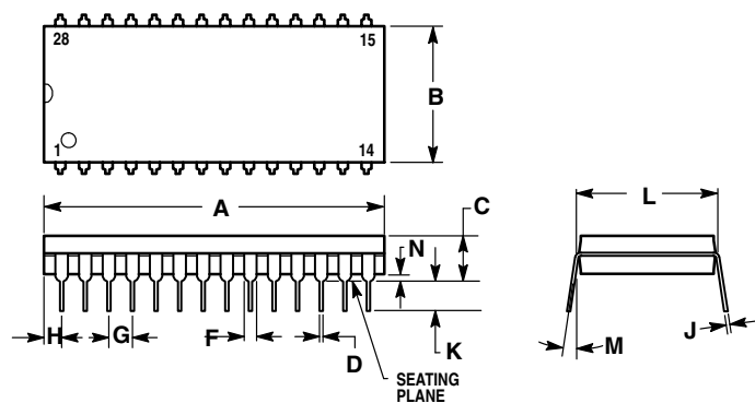
Figure 18-3. 28-Pin PDIP (Case #710)
