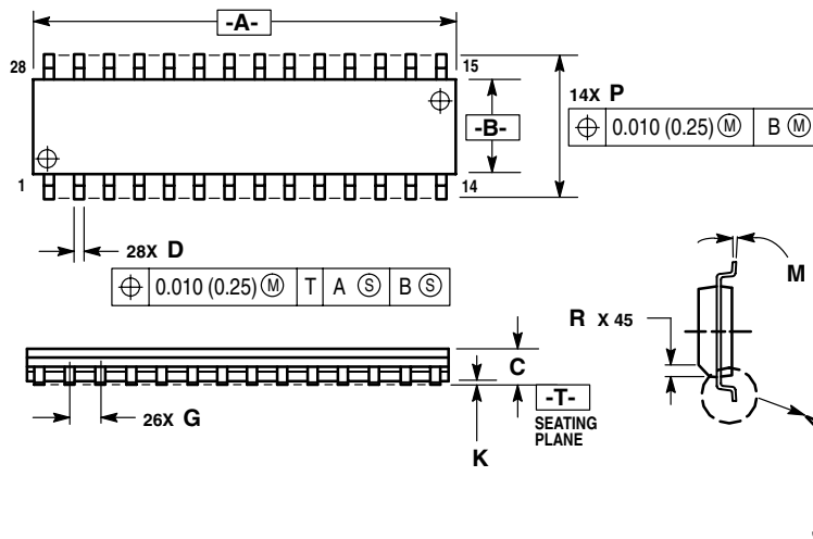
Figure 18-4. 28-Pin SOIC (Case #751F)
