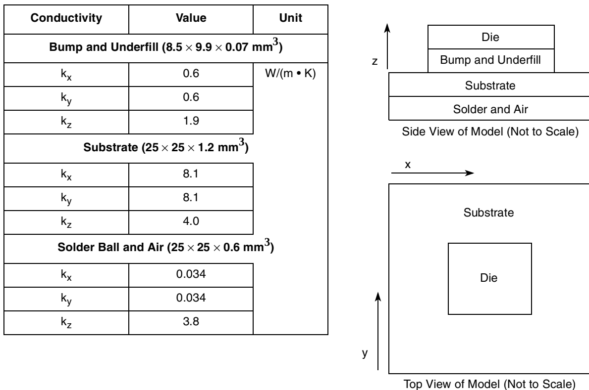
Figure 24. Recommended Thermal Model of MPC7447A
