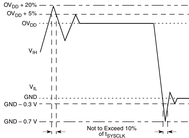
Figure 2. Overshoot/Undershoot Voltage
