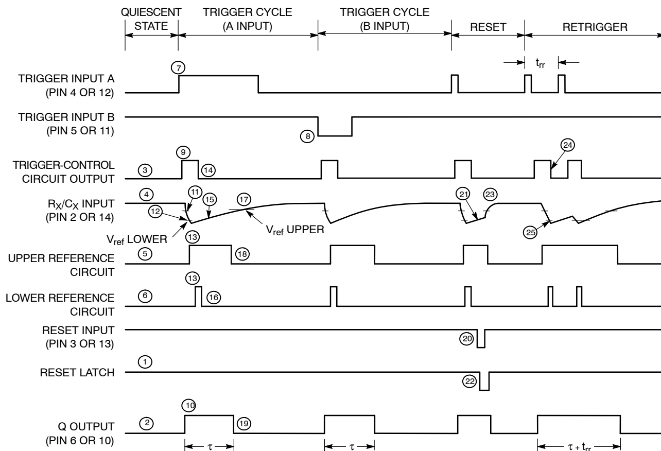
Figure 12. Timing Diagram
