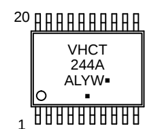
1 TSSOP-20 SUFFIX DT CASE 948E
