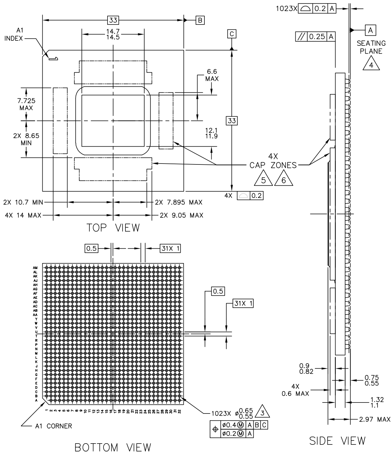
Figure 57. MPC8641D High-Head FC-CBGA Dimensions
