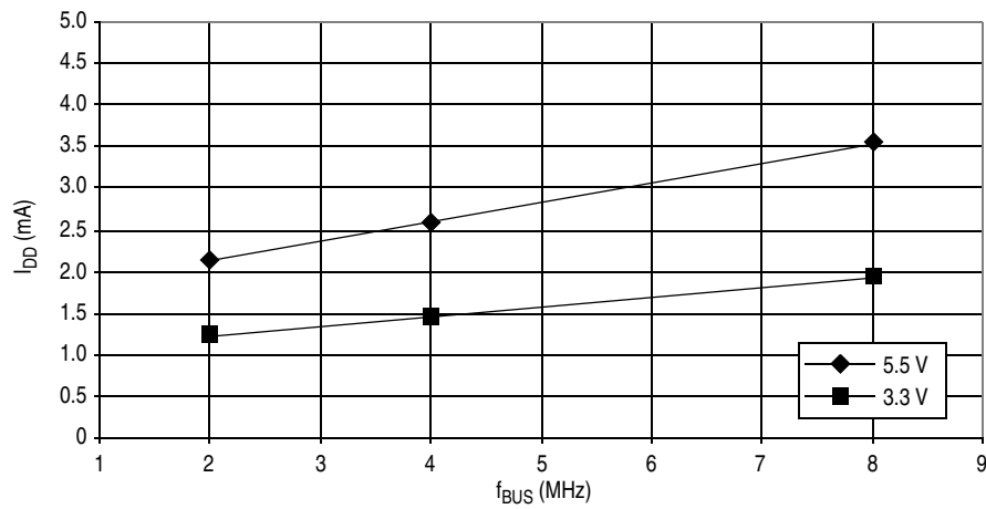
Figure 20-15. Typical Wait Mode I DD
