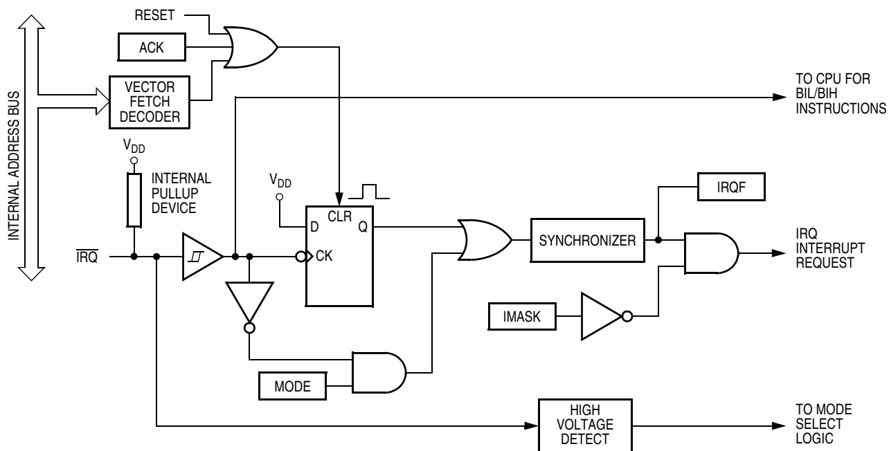
Figure 7-1. IRQ Module Block Diagram
