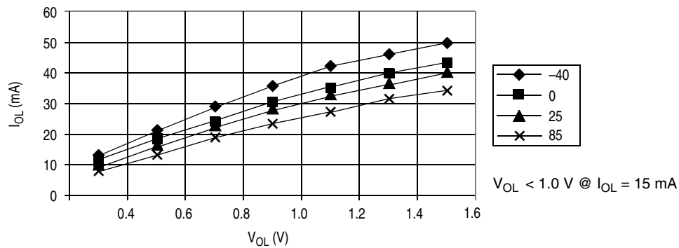
Figure 20-10. Typical Low-Side Driver Characteristics — Port PTC4–PTC0 ( V_{DD} = 4.5 \text{ Vdc} )
