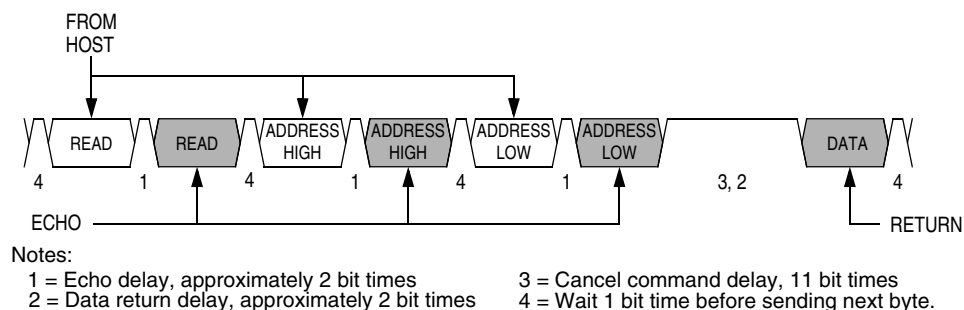
Figure 19-12. Read Transaction
