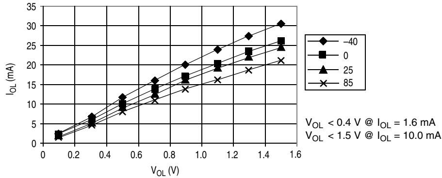
Figure 20-8. Typical Low-Side Driver Characteristics — Port PTA7–PTA0 ( V_{DD} = 5.5 \text{ Vdc} )
