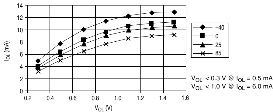
Figure 20-9. Typical Low-Side Driver Characteristics — Port PTA7–PTA0 ( V_{DD} = 2.7 \text{ Vdc} )
