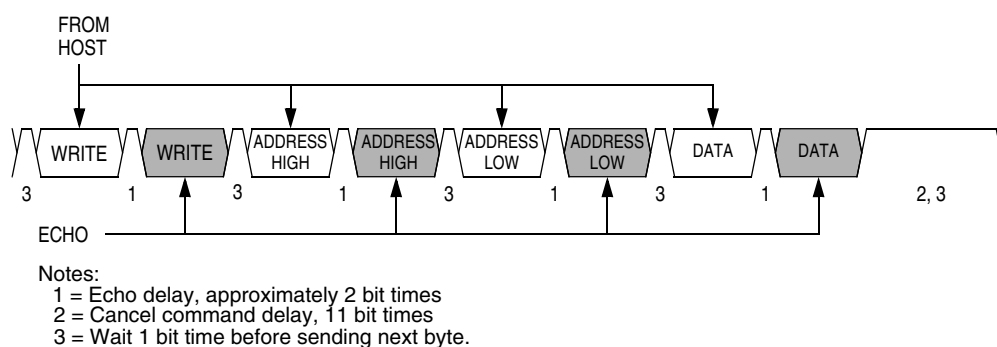
Figure 19-13. Write Transaction
