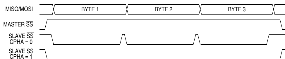
Figure 16-6. CPHA/\overline{SS} Timing
