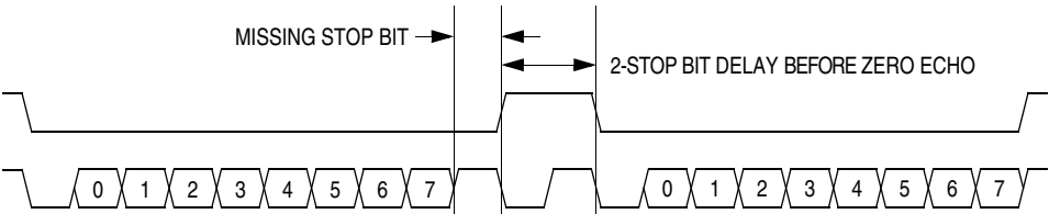
Figure 19-11. Break Transaction
