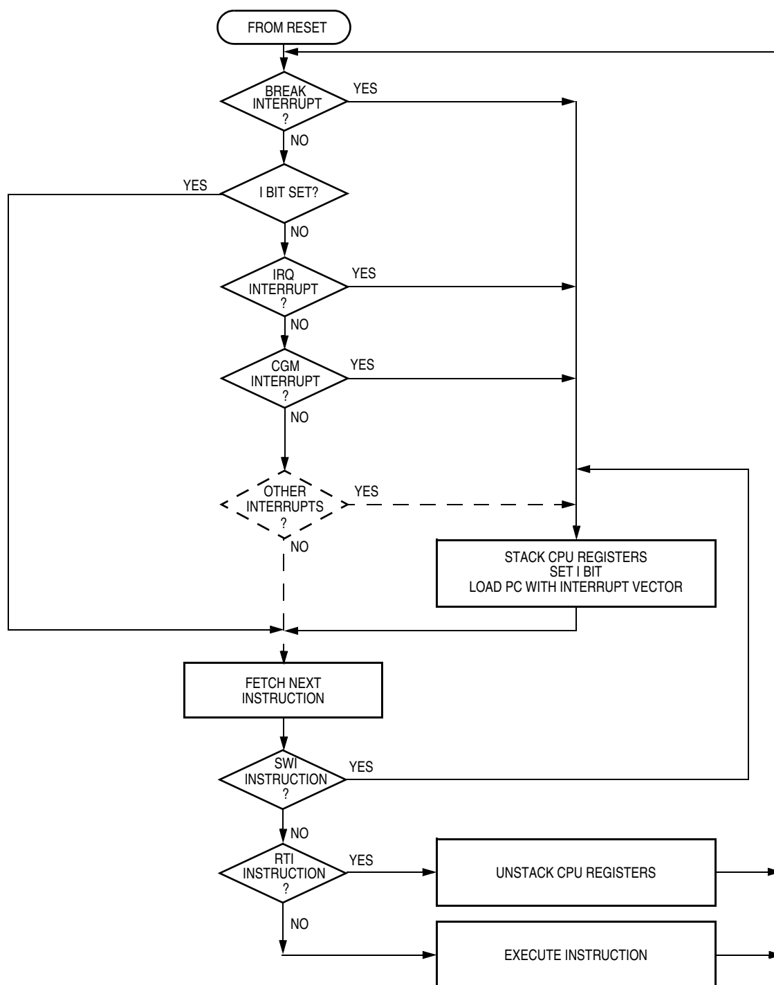
Figure 13-6. Interrupt Processing
