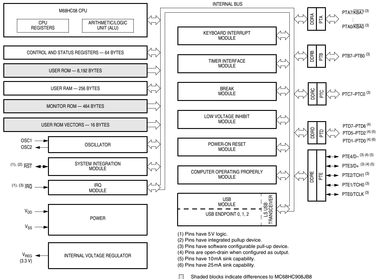
Figure A-1. MC68HC08JB8 Block Diagram
