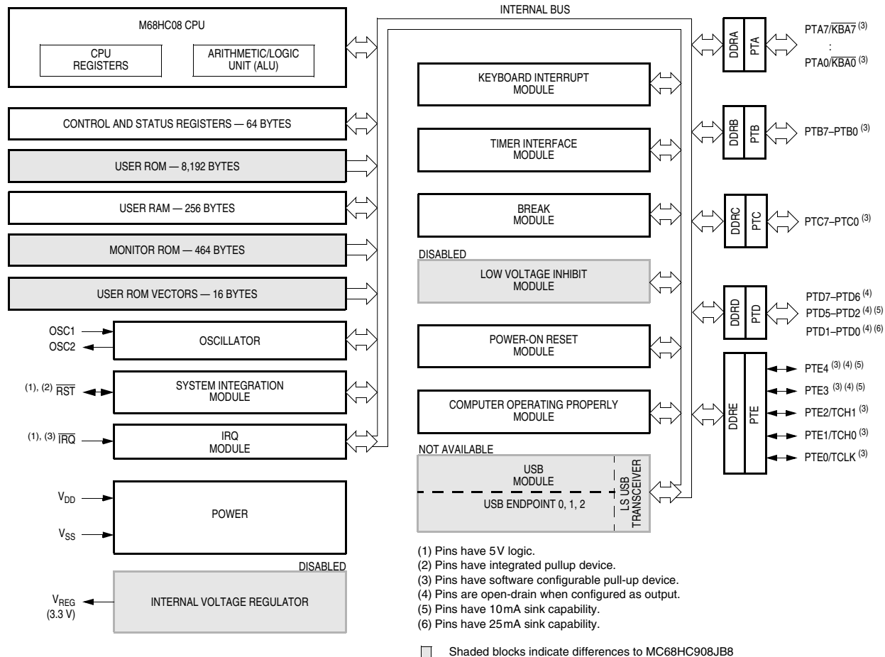
Figure B-1. MC68HC08JT8 Block Diagram
