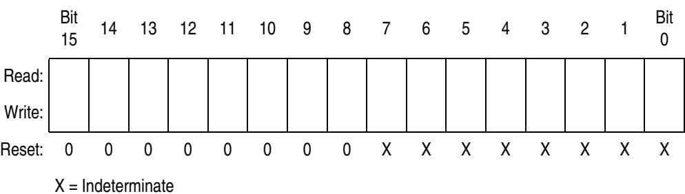
Figure 6-3. Index Register (H:X)
