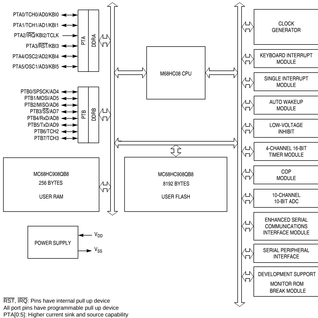
Figure 1-1. Block Diagram
