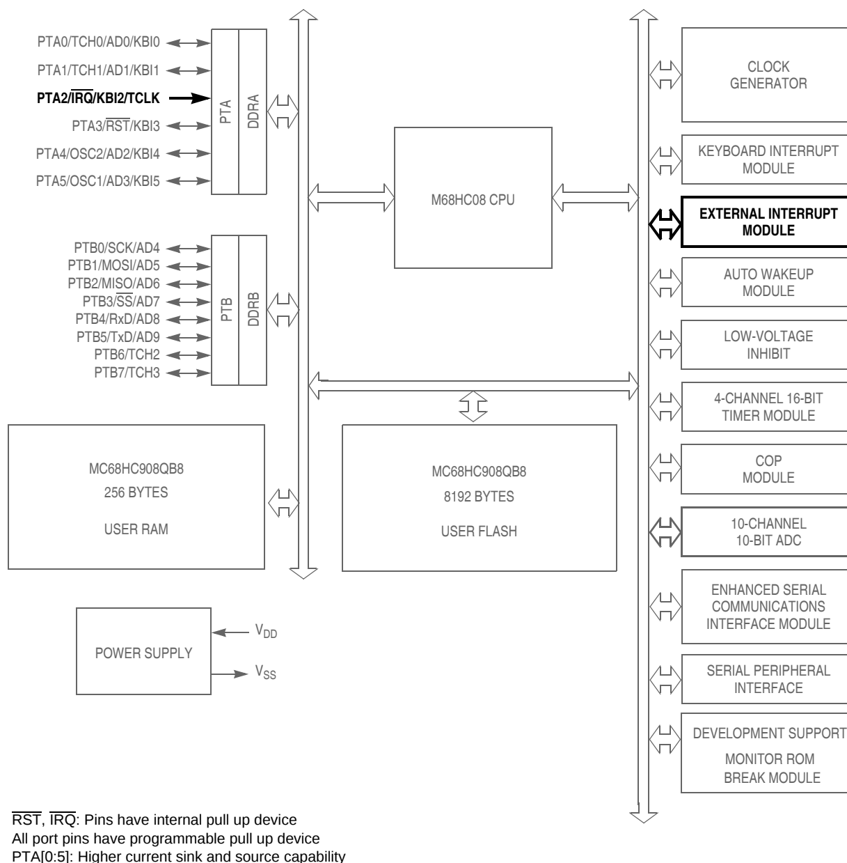
Figure 8-1. Block Diagram Highlighting IRQ Block and Pin
